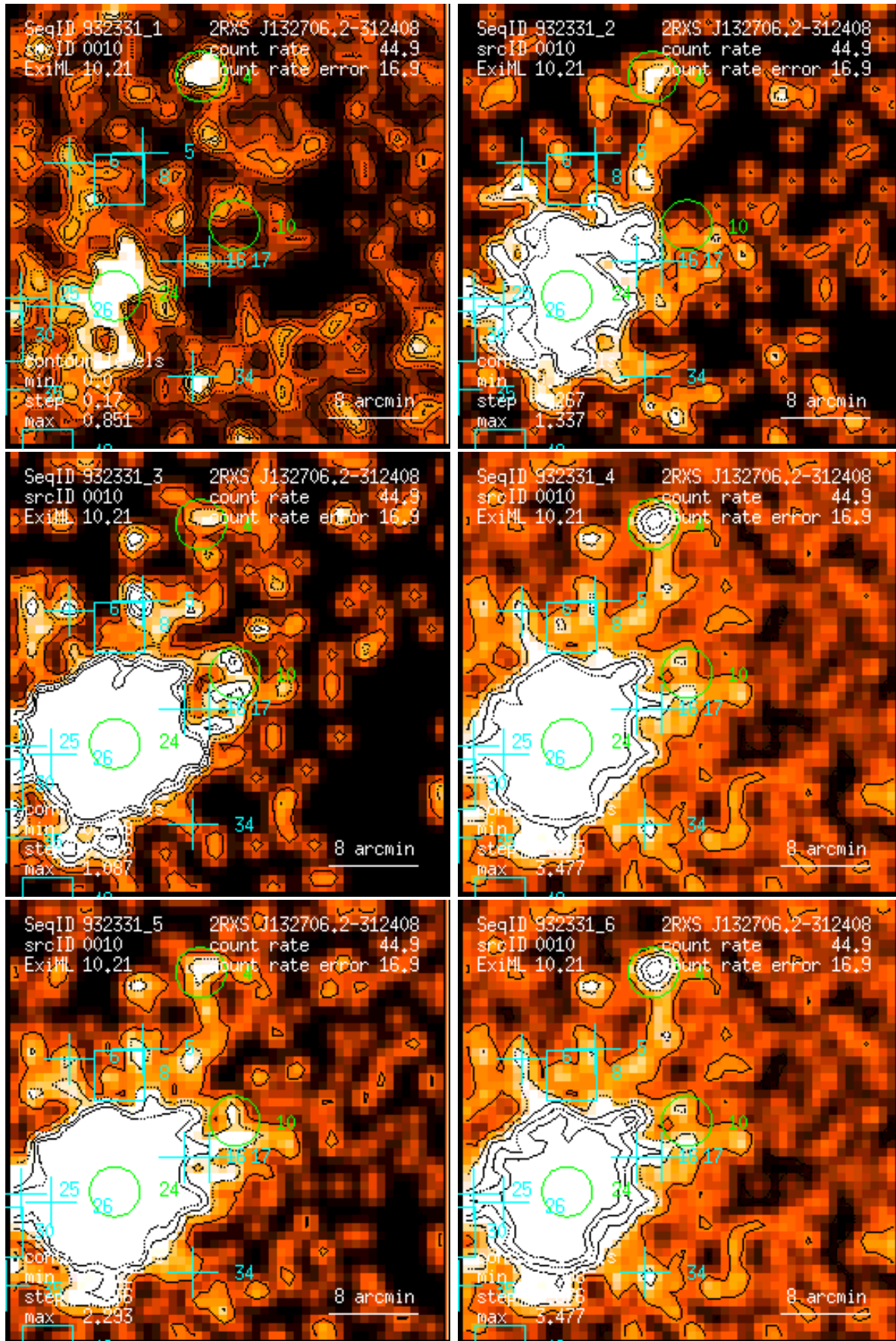
Figure 10: RASS 932331: detection 0010: band rate images, Gaussian filter: (1) PSPC channels 11 – 41, (2) 52 – 90, (3) 91 – 201, (4) 11 – 235, (5) 52 – 201, (6) 11 – 201. Broad band rates in counts/ks. Band rate contour levels in counts/ks/arcmin 2 .
