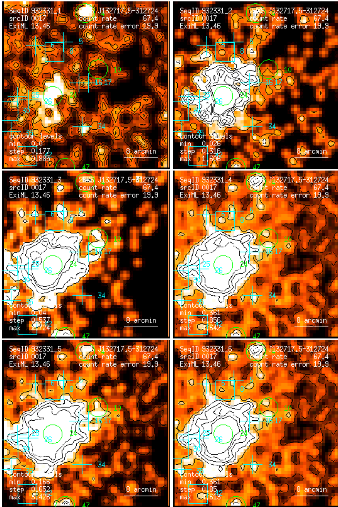
Figure 17: RASS 932331: detection 0017: band rate images, Gaussian filter: (1) PSPC channels 11 – 41, (2) 52 – 90, (3) 91 – 201, (4) 11 – 235, (5) 52 – 201, (6) 11 – 201. Broad band rates in counts/ks. Band rate contour levels in counts/ks/arcmin 2 .
