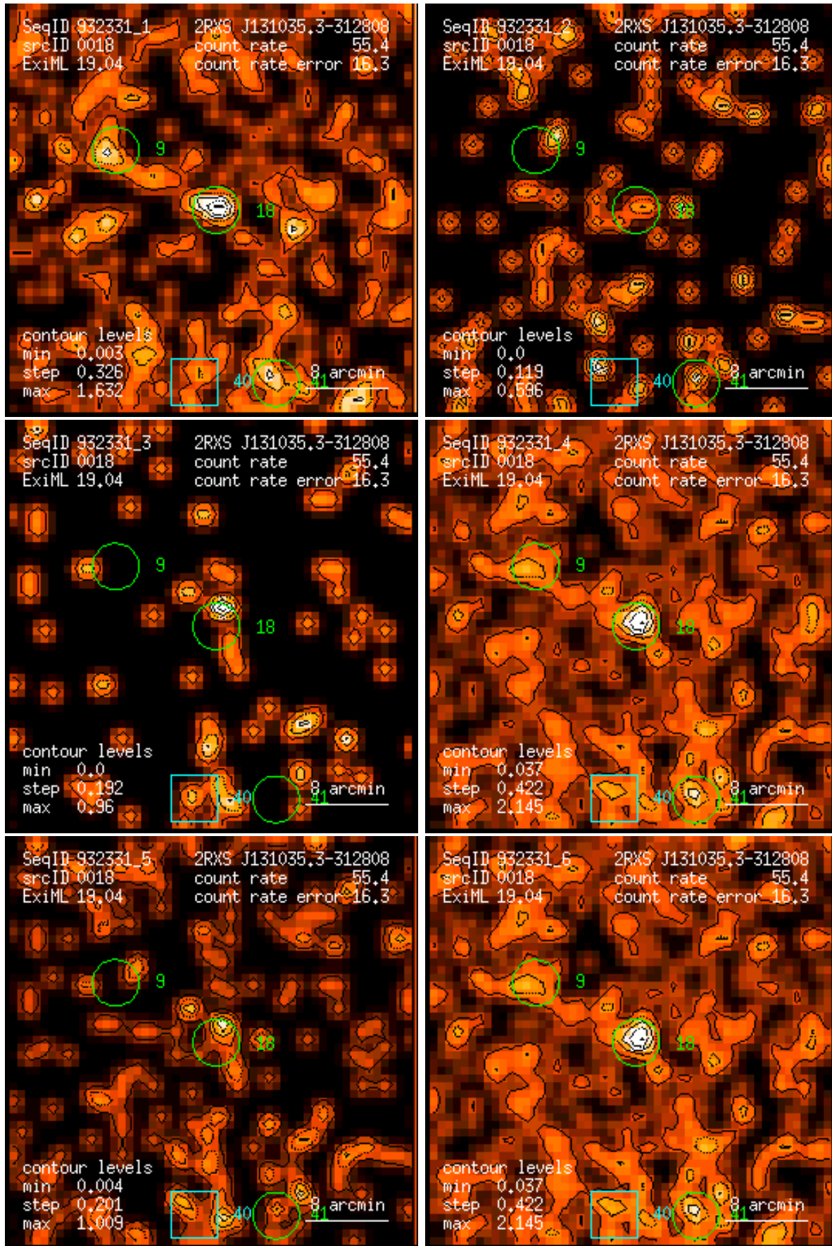
Figure 18: RASS 932331: detection 0018: band rate images, Gaussian filter: (1) PSPC channels 11 – 41, (2) 52 – 90, (3) 91 – 201, (4) 11 – 235, (5) 52 – 201, (6) 11 – 201. Broad band rates in counts/ks. Band rate contour levels in counts/ks/arcmin 2 .
