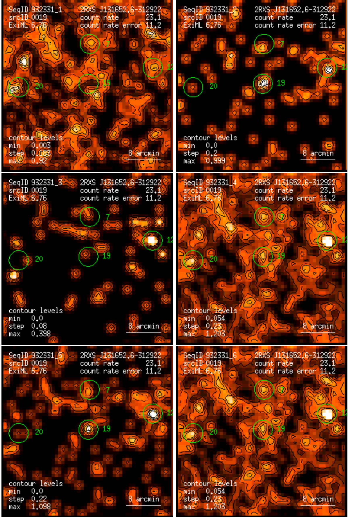
Figure 19: RASS 932331: detection 0019: band rate images, Gaussian filter: (1) PSPC channels 11 – 41, (2) 52 – 90, (3) 91 – 201, (4) 11 – 235, (5) 52 – 201, (6) 11 – 201. Broad band rates in counts/ks. Band rate contour levels in counts/ks/arcmin 2 .
