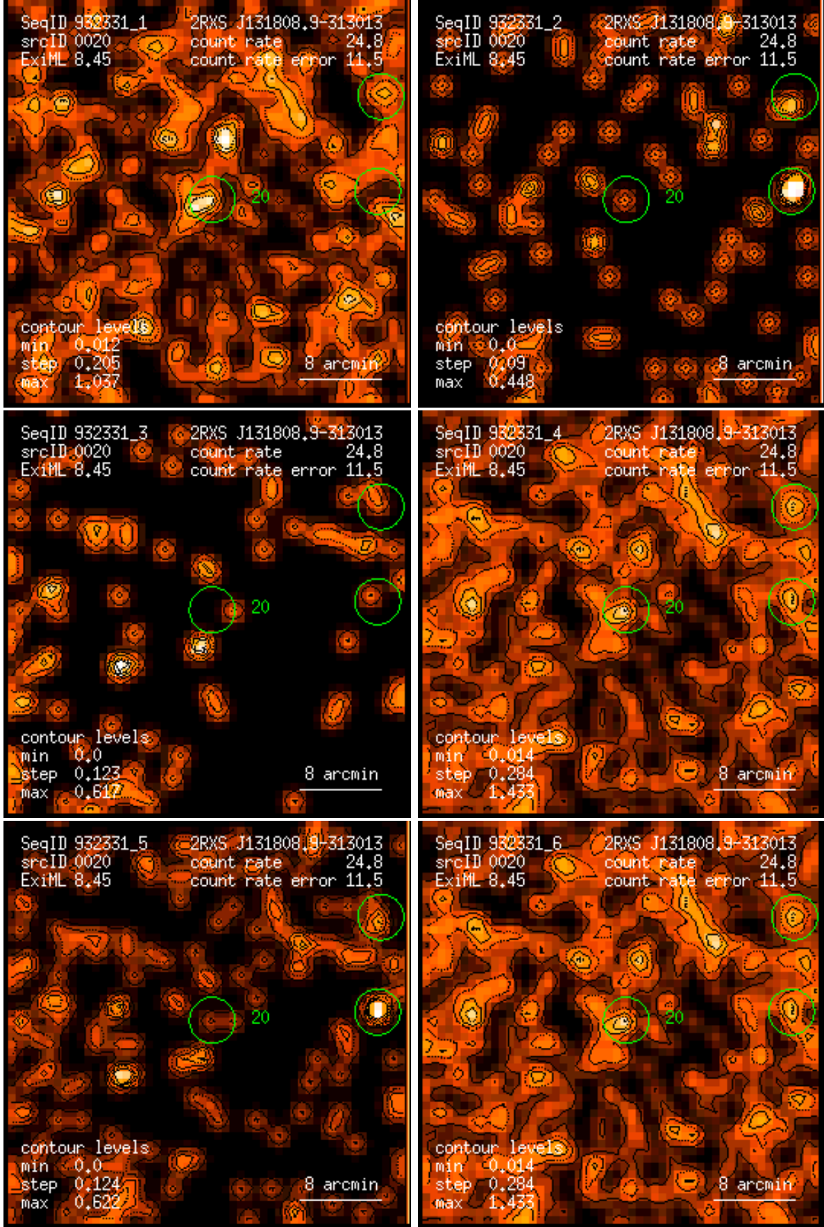
Figure 20: RASS 932331: detection 0020: band rate images, Gaussian filter: (1) PSPC channels 11 – 41, (2) 52 – 90, (3) 91 – 201, (4) 11 – 235, (5) 52 – 201, (6) 11 – 201. Broad band rates in counts/ks. Band rate contour levels in counts/ks/arcmin 2 .
