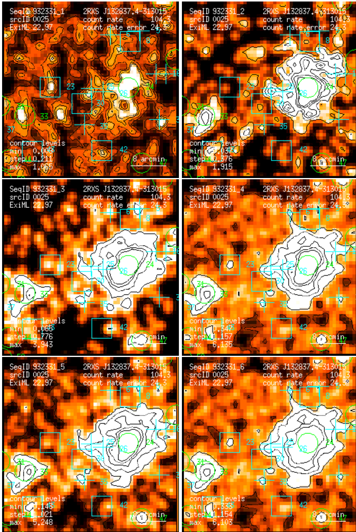
Figure 25: RASS 932331: detection 0025: band rate images, Gaussian filter: (1) PSPC channels 11 – 41, (2) 52 – 90, (3) 91 – 201, (4) 11 – 235, (5) 52 – 201, (6) 11 – 201. Broad band rates in counts/ks. Band rate contour levels in counts/ks/arcmin 2 .
