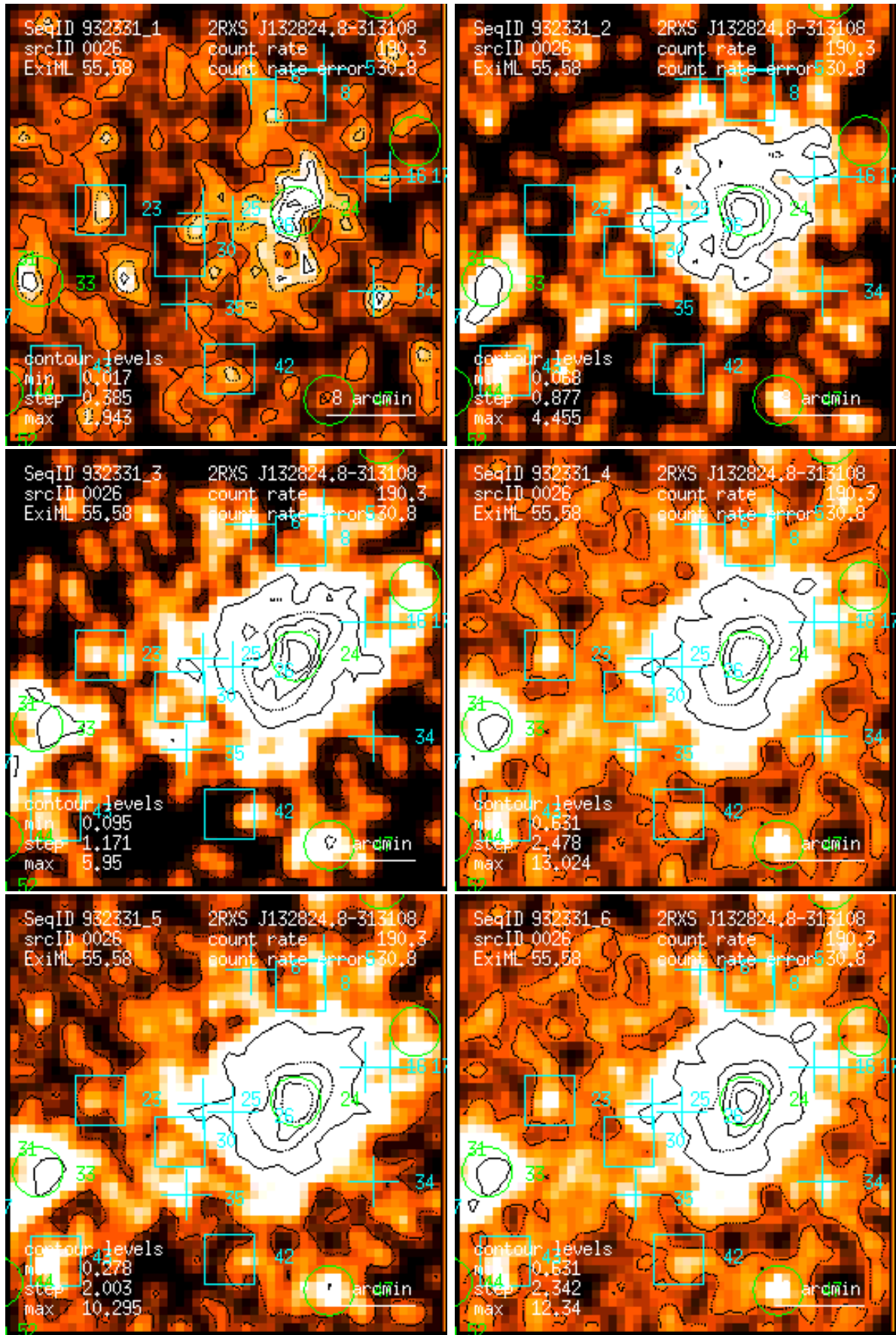
Figure 26: RASS 932331: detection 0026: band rate images, Gaussian filter: (1) PSPC channels 11 – 41, (2) 52 – 90, (3) 91 – 201, (4) 11 – 235, (5) 52 – 201, (6) 11 – 201. Broad band rates in counts/ks. Band rate contour levels in counts/ks/arcmin 2 .
