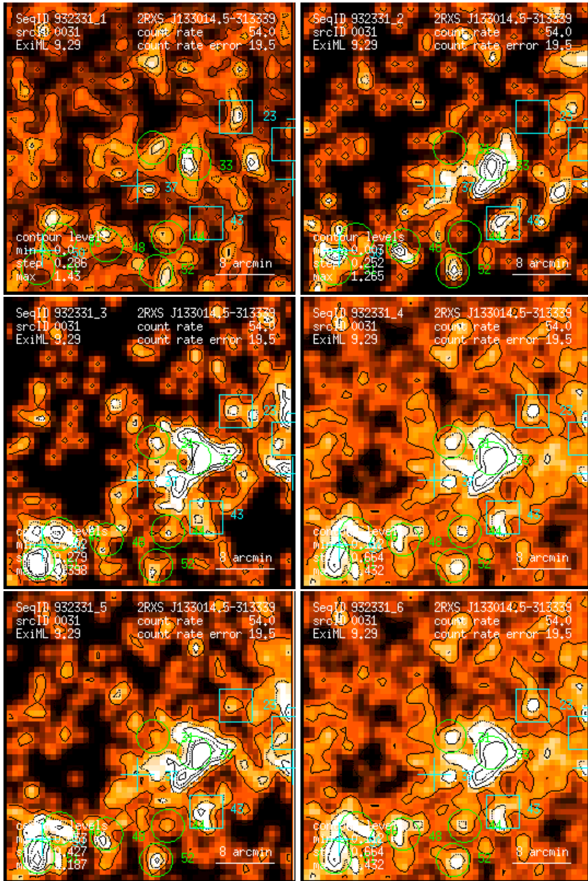
Figure 31: RASS 932331: detection 0031: band rate images, Gaussian filter: (1) PSPC channels 11 – 41, (2) 52 – 90, (3) 91 – 201, (4) 11 – 235, (5) 52 – 201, (6) 11 – 201. Broad band rates in counts/ks. Band rate contour levels in counts/ks/arcmin 2 .
