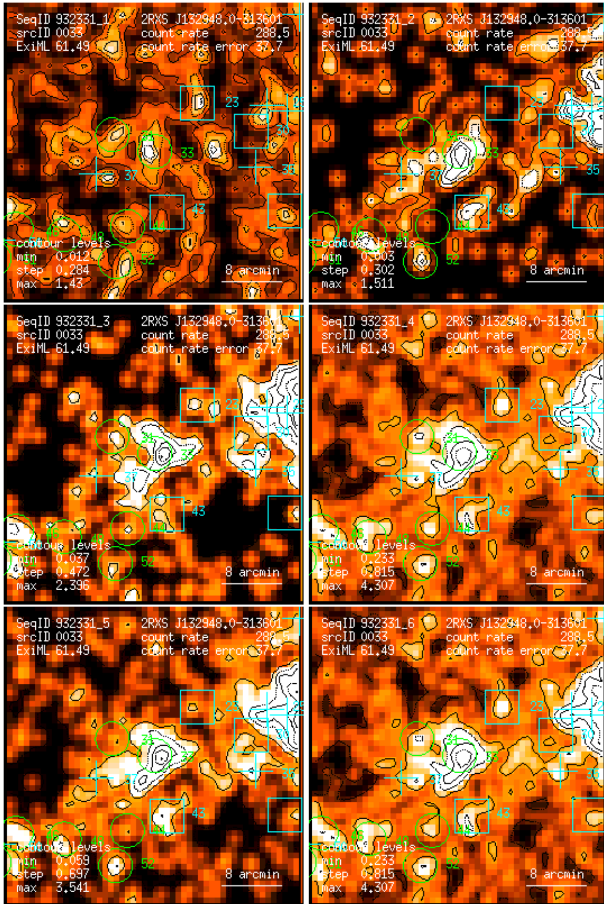
Figure 33: RASS 932331: detection 0033: band rate images, Gaussian filter: (1) PSPC channels 11 – 41, (2) 52 – 90, (3) 91 – 201, (4) 11 – 235, (5) 52 – 201, (6) 11 – 201. Broad band rates in counts/ks. Band rate contour levels in counts/ks/arcmin 2 .
