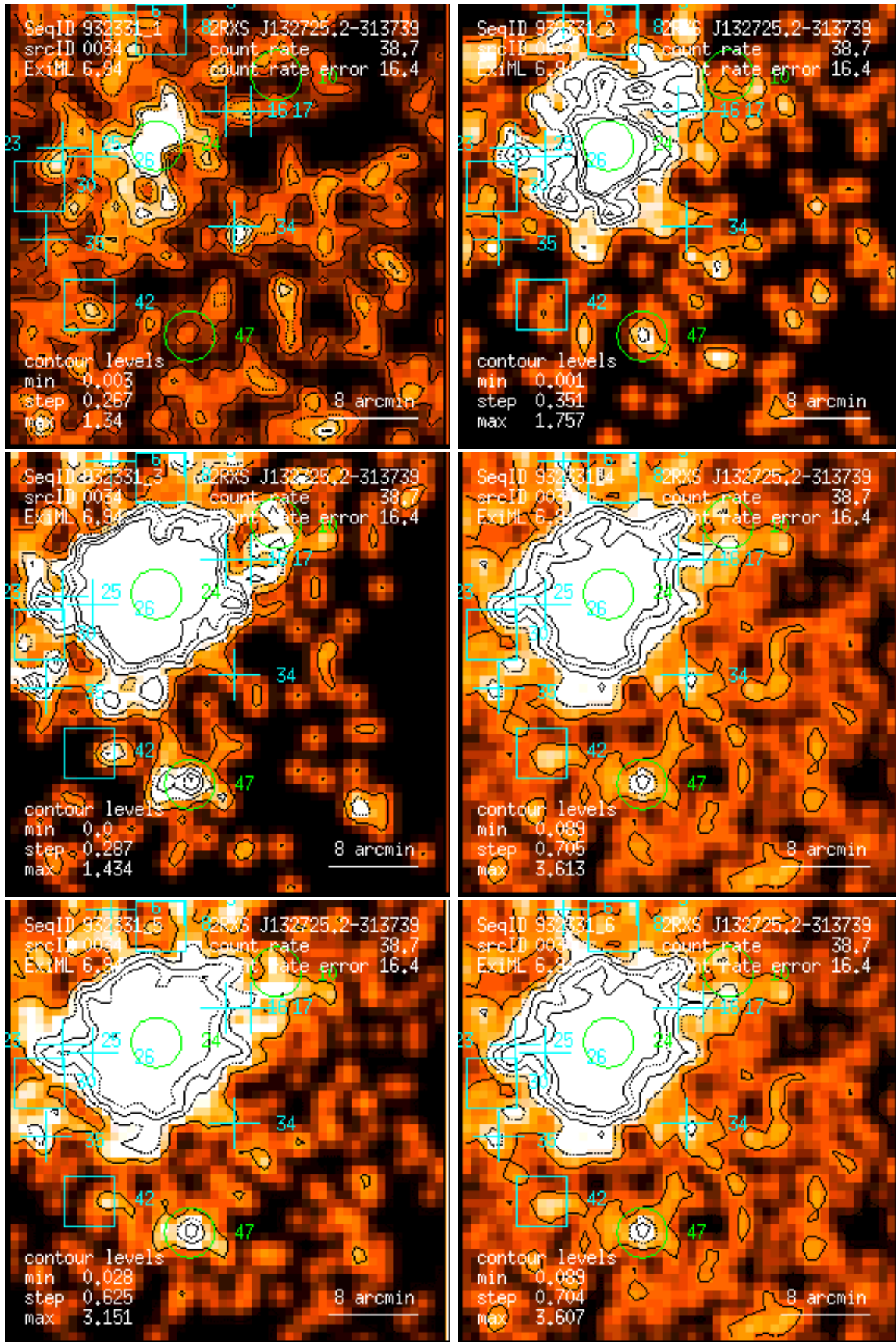
Figure 34: RASS 932331: detection 0034: band rate images, Gaussian filter: (1) PSPC channels 11 – 41, (2) 52 – 90, (3) 91 – 201, (4) 11 – 235, (5) 52 – 201, (6) 11 – 201. Broad band rates in counts/ks. Band rate contour levels in counts/ks/arcmin 2 .
