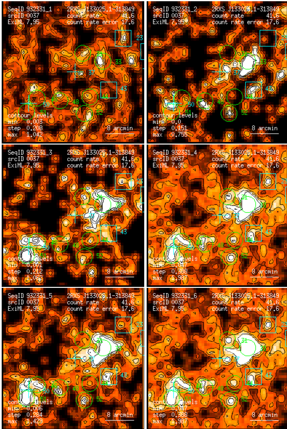
Figure 37: RASS 932331: detection 0037: band rate images, Gaussian filter: (1) PSPC channels 11 – 41, (2) 52 – 90, (3) 91 – 201, (4) 11 – 235, (5) 52 – 201, (6) 11 – 201. Broad band rates in counts/ks. Band rate contour levels in counts/ks/arcmin 2 .
