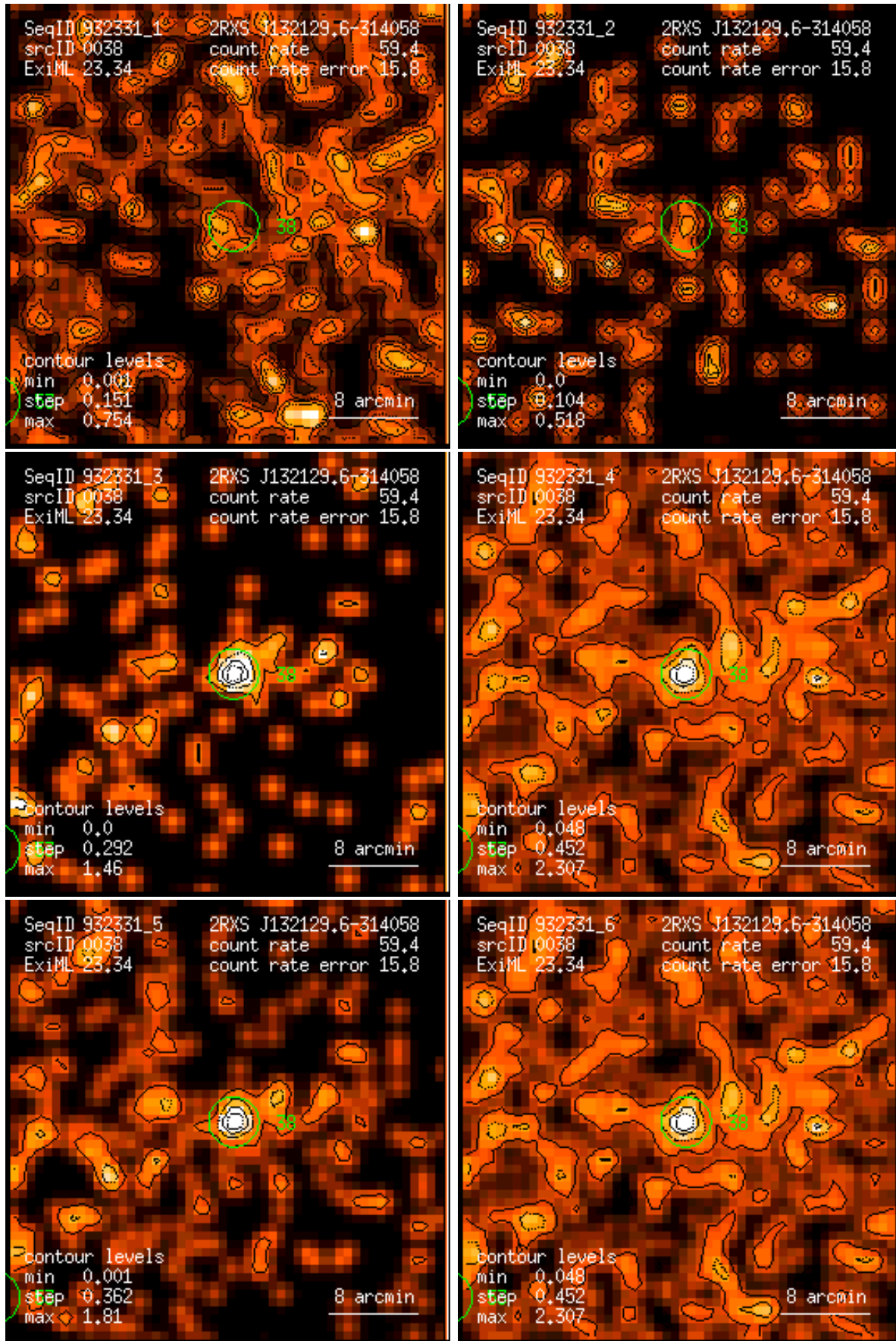
Figure 38: RASS 932331: detection 0038: band rate images, Gaussian filter: (1) PSPC channels 11 – 41, (2) 52 – 90, (3) 91 – 201, (4) 11 – 235, (5) 52 – 201, (6) 11 – 201. Broad band rates in counts/ks. Band rate contour levels in counts/ks/arcmin 2 .
