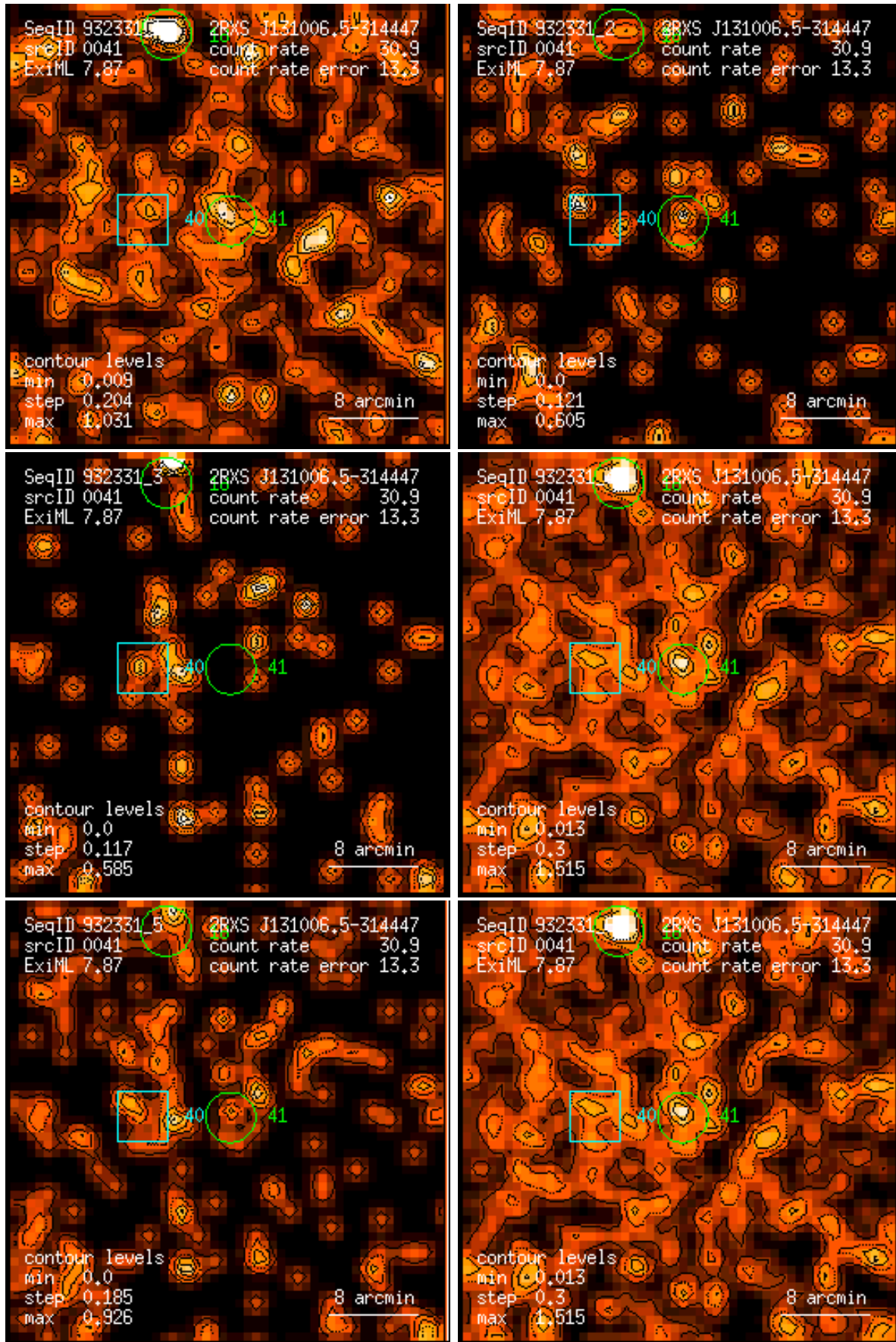
Figure 41: RASS 932331: detection 0041: band rate images, Gaussian filter: (1) PSPC channels 11 – 41, (2) 52 – 90, (3) 91 – 201, (4) 11 – 235, (5) 52 – 201, (6) 11 – 201. Broad band rates in counts/ks. Band rate contour levels in counts/ks/arcmin 2 .
