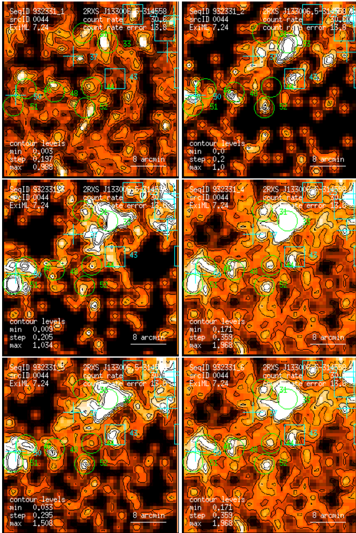
Figure 44: RASS 932331: detection 0044: band rate images, Gaussian filter: (1) PSPC channels 11 – 41, (2) 52 – 90, (3) 91 – 201, (4) 11 – 235, (5) 52 – 201, (6) 11 – 201. Broad band rates in counts/ks. Band rate contour levels in counts/ks/arcmin 2 .
