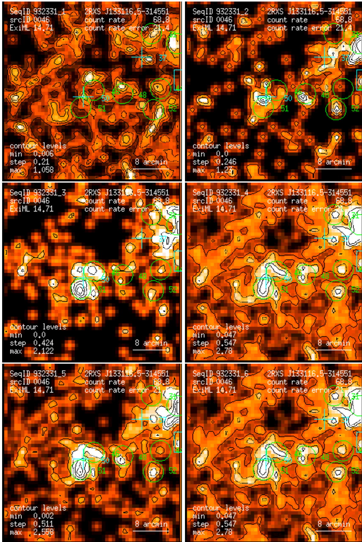
Figure 46: RASS 932331: detection 0046: band rate images, Gaussian filter: (1) PSPC channels 11 – 41, (2) 52 – 90, (3) 91 – 201, (4) 11 – 235, (5) 52 – 201, (6) 11 – 201. Broad band rates in counts/ks. Band rate contour levels in counts/ks/arcmin 2 .
