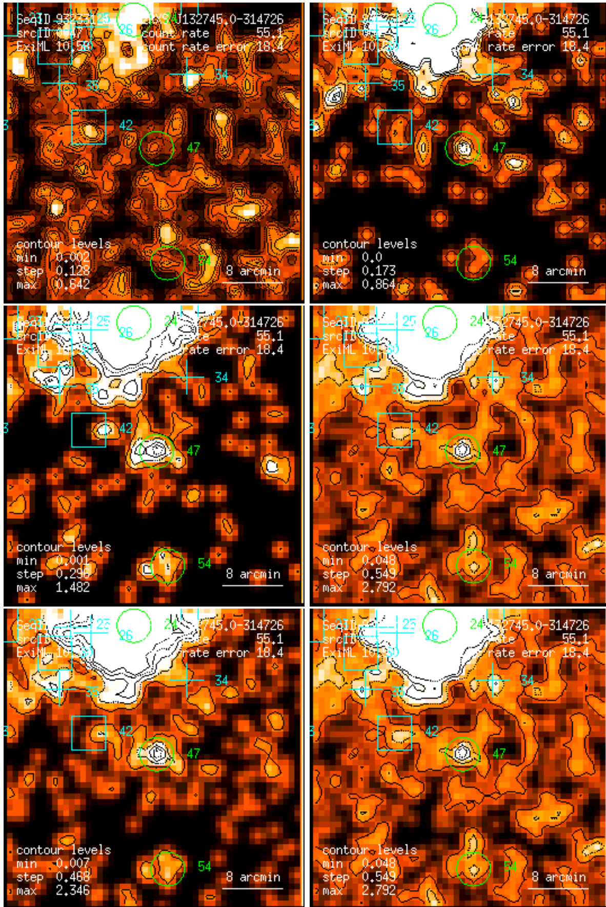
Figure 47: RASS 932331: detection 0047: band rate images, Gaussian filter: (1) PSPC channels 11 – 41, (2) 52 – 90, (3) 91 – 201, (4) 11 – 235, (5) 52 – 201, (6) 11 – 201. Broad band rates in counts/ks. Band rate contour levels in counts/ks/arcmin 2 .
