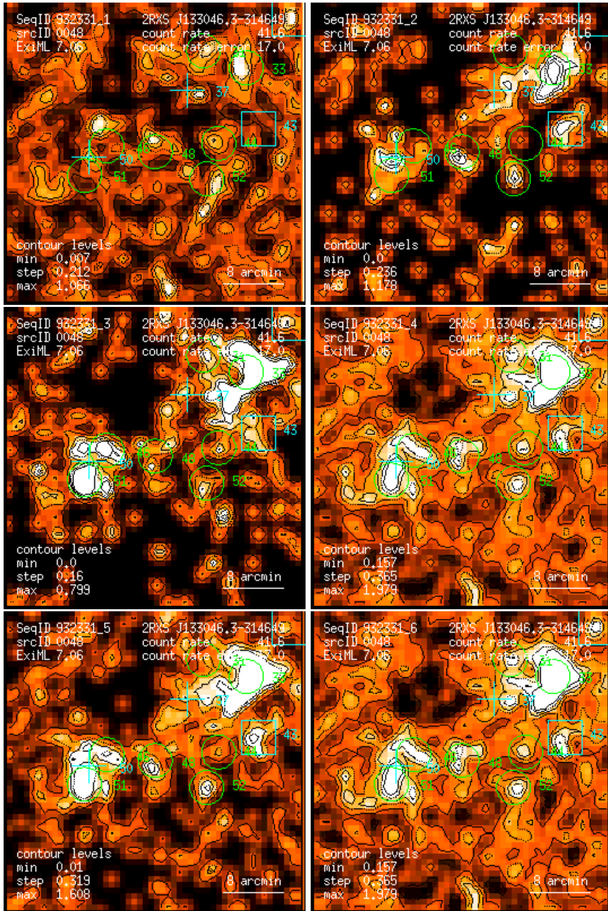
Figure 48: RASS 932331: detection 0048: band rate images, Gaussian filter: (1) PSPC channels 11 – 41, (2) 52 – 90, (3) 91 – 201, (4) 11 – 235, (5) 52 – 201, (6) 11 – 201. Broad band rates in counts/ks. Band rate contour levels in counts/ks/arcmin 2 .
