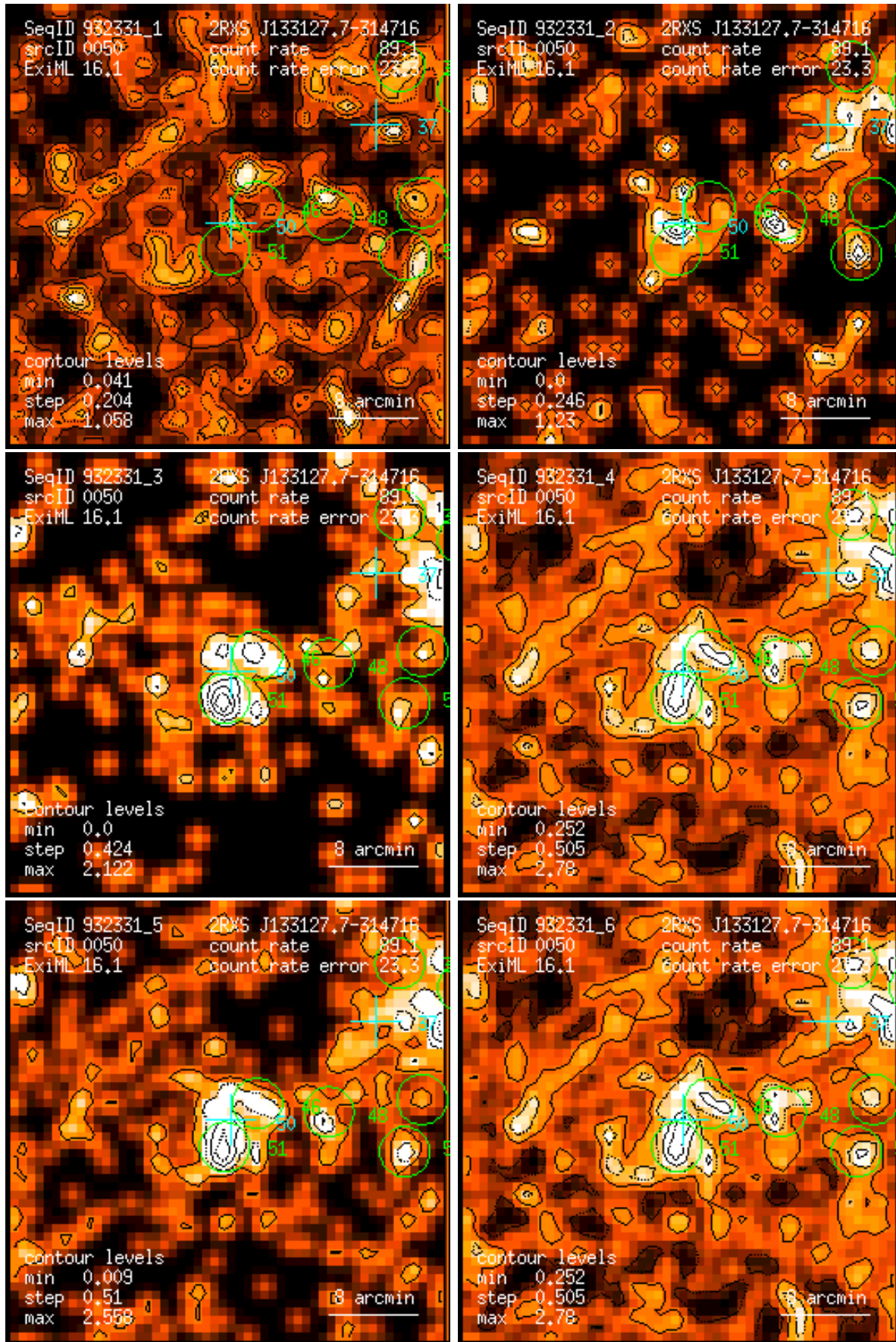
Figure 50: RASS 932331: detection 0050: band rate images, Gaussian filter: (1) PSPC channels 11 – 41, (2) 52 – 90, (3) 91 – 201, (4) 11 – 235, (5) 52 – 201, (6) 11 – 201. Broad band rates in counts/ks. Band rate contour levels in counts/ks/arcmin 2 .
