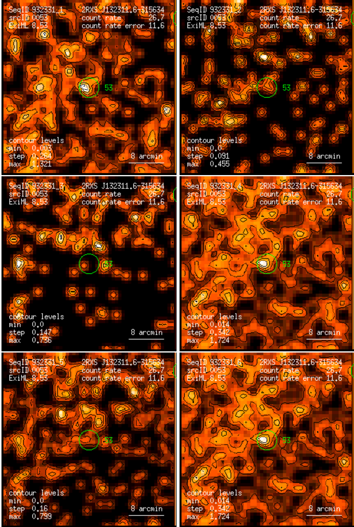
Figure 53: RASS 932331: detection 0053: band rate images, Gaussian filter: (1) PSPC channels 11 – 41, (2) 52 – 90, (3) 91 – 201, (4) 11 – 235, (5) 52 – 201, (6) 11 – 201. Broad band rates in counts/ks. Band rate contour levels in counts/ks/arcmin 2 .
