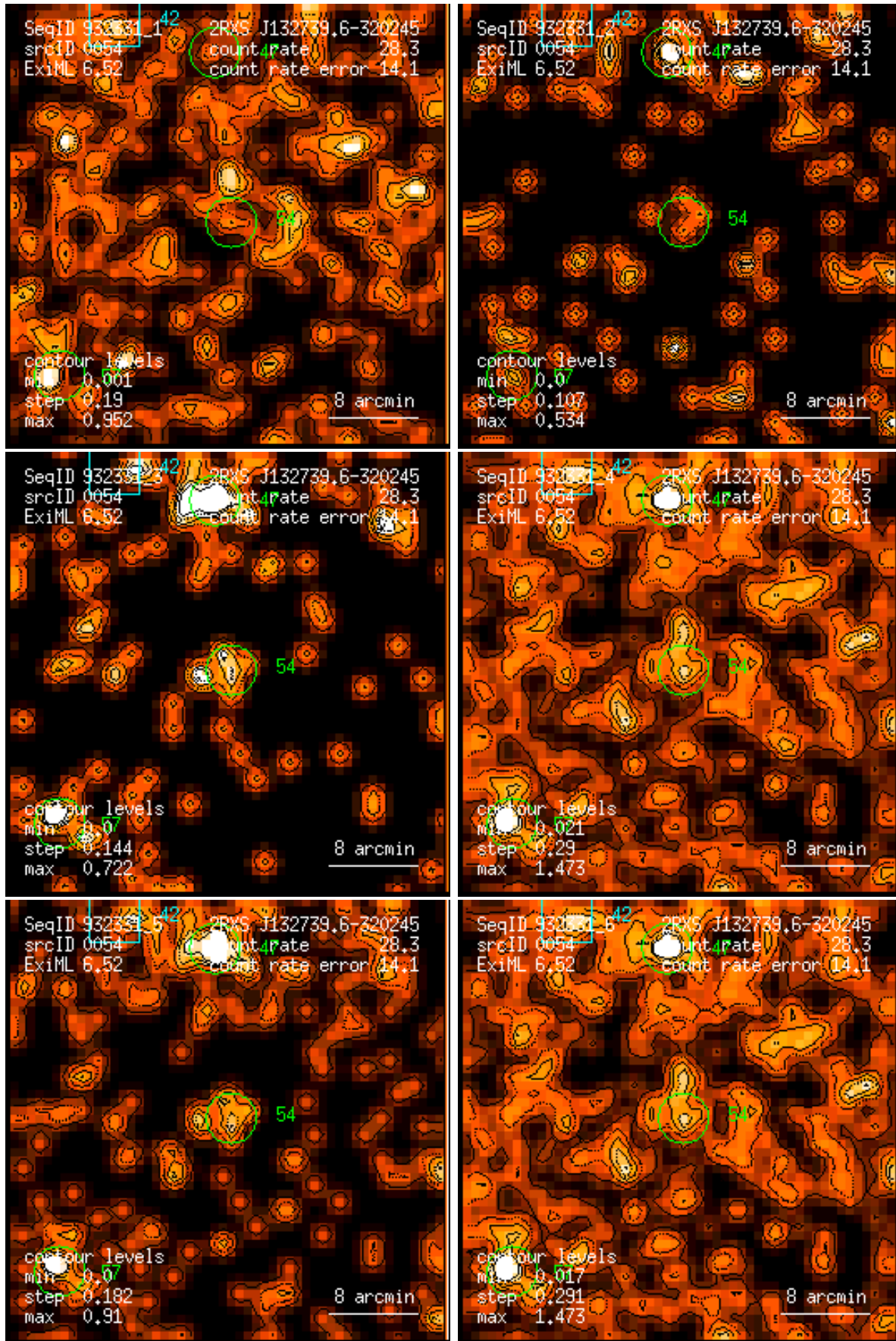
Figure 54: RASS 932331: detection 0054: band rate images, Gaussian filter: (1) PSPC channels 11 – 41, (2) 52 – 90, (3) 91 – 201, (4) 11 – 235, (5) 52 – 201, (6) 11 – 201. Broad band rates in counts/ks. Band rate contour levels in counts/ks/arcmin 2 .
