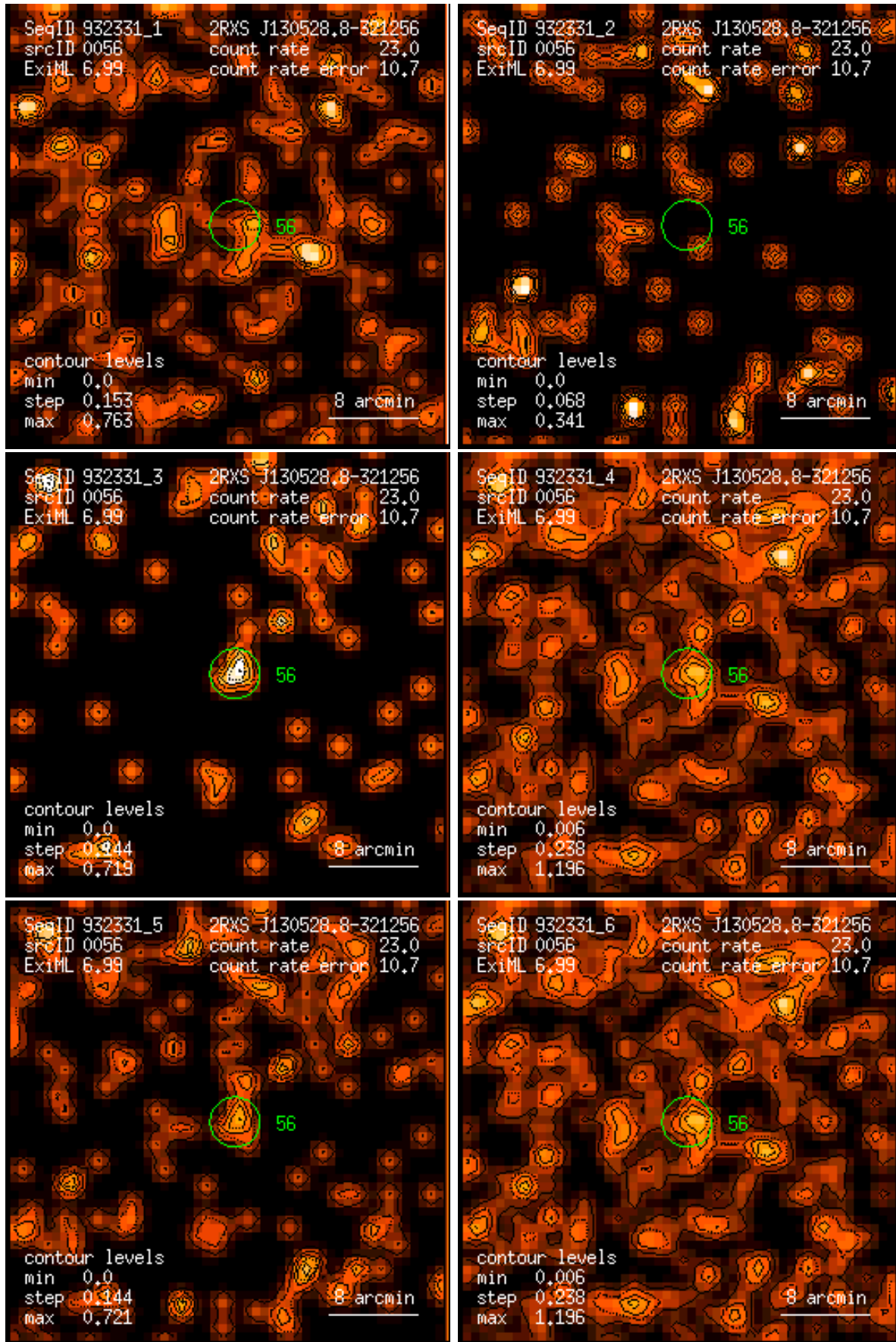
Figure 56: RASS 932331: detection 0056: band rate images, Gaussian filter: (1) PSPC channels 11 – 41, (2) 52 – 90, (3) 91 – 201, (4) 11 – 235, (5) 52 – 201, (6) 11 – 201. Broad band rates in counts/ks. Band rate contour levels in counts/ks/arcmin 2 .
