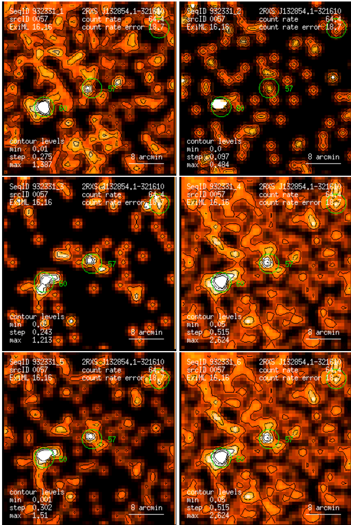
Figure 57: RASS 932331: detection 0057: band rate images, Gaussian filter: (1) PSPC channels 11 – 41, (2) 52 – 90, (3) 91 – 201, (4) 11 – 235, (5) 52 – 201, (6) 11 – 201. Broad band rates in counts/ks. Band rate contour levels in counts/ks/arcmin 2 .
