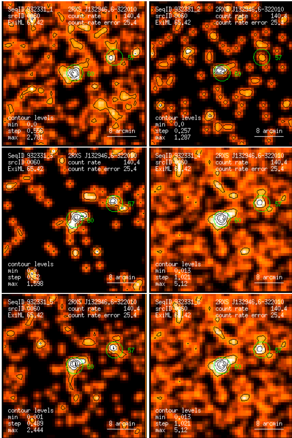
Figure 60: RASS 932331: detection 0060: band rate images, Gaussian filter: (1) PSPC channels 11 – 41, (2) 52 – 90, (3) 91 – 201, (4) 11 – 235, (5) 52 – 201, (6) 11 – 201. Broad band rates in counts/ks. Band rate contour levels in counts/ks/arcmin 2 .
