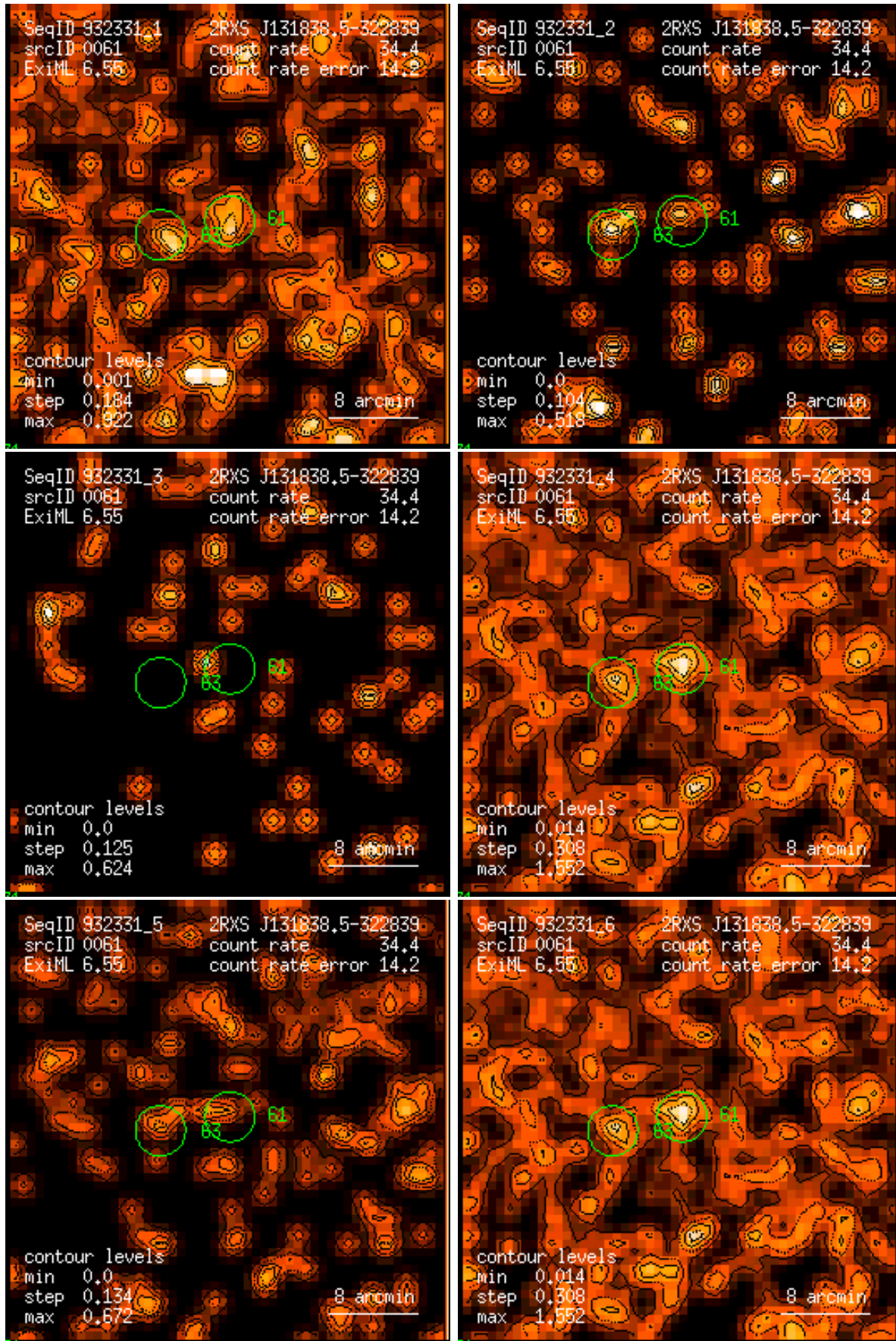
Figure 61: RASS 932331: detection 0061: band rate images, Gaussian filter: (1) PSPC channels 11 – 41, (2) 52 – 90, (3) 91 – 201, (4) 11 – 235, (5) 52 – 201, (6) 11 – 201. Broad band rates in counts/ks. Band rate contour levels in counts/ks/arcmin 2 .
