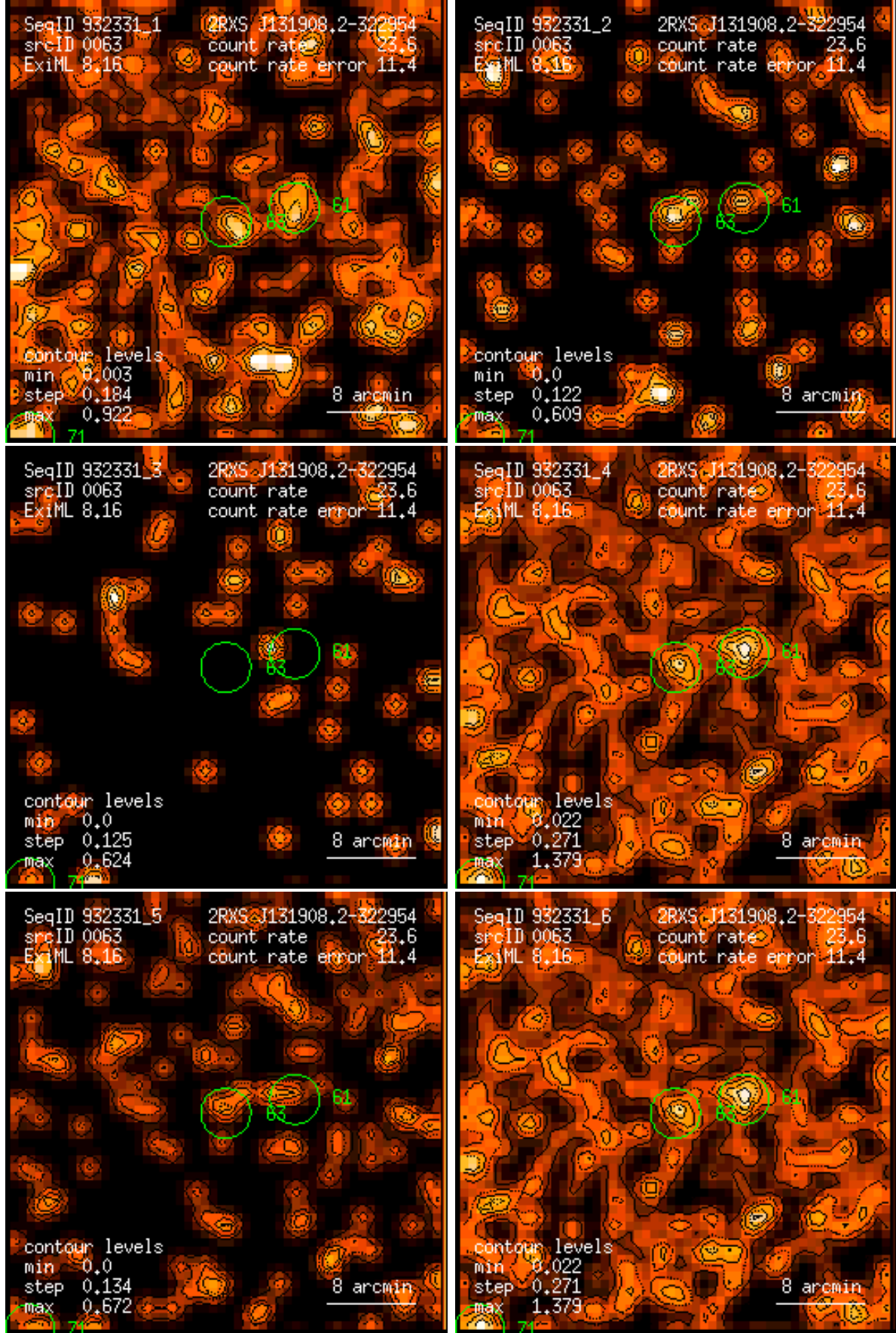
Figure 63: RASS 932331: detection 0063: band rate images, Gaussian filter: (1) PSPC channels 11 – 41, (2) 52 – 90, (3) 91 – 201, (4) 11 – 235, (5) 52 – 201, (6) 11 – 201. Broad band rates in counts/ks. Band rate contour levels in counts/ks/arcmin 2 .
