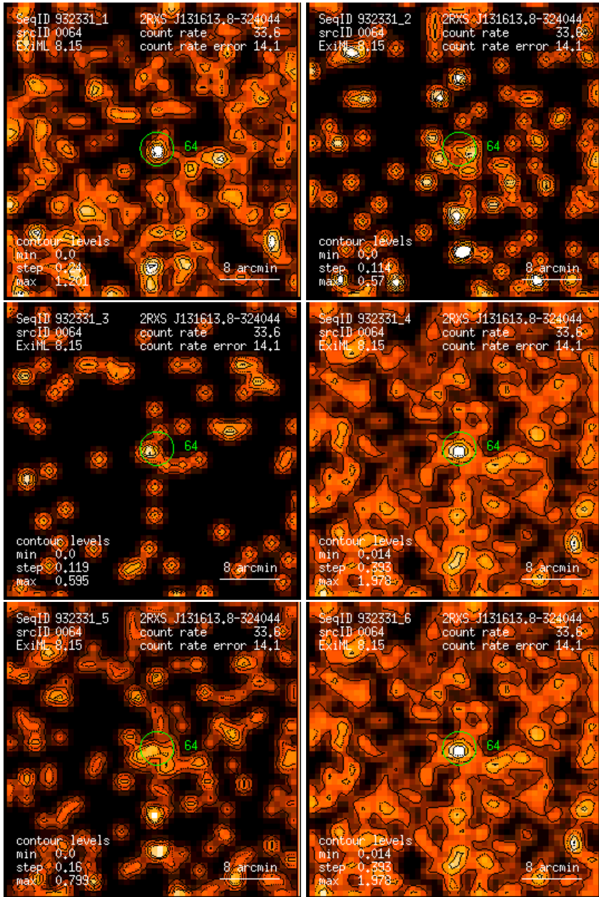
Figure 64: RASS 932331: detection 0064: band rate images, Gaussian filter: (1) PSPC channels 11 – 41, (2) 52 – 90, (3) 91 – 201, (4) 11 – 235, (5) 52 – 201, (6) 11 – 201. Broad band rates in counts/ks. Band rate contour levels in counts/ks/arcmin 2 .
