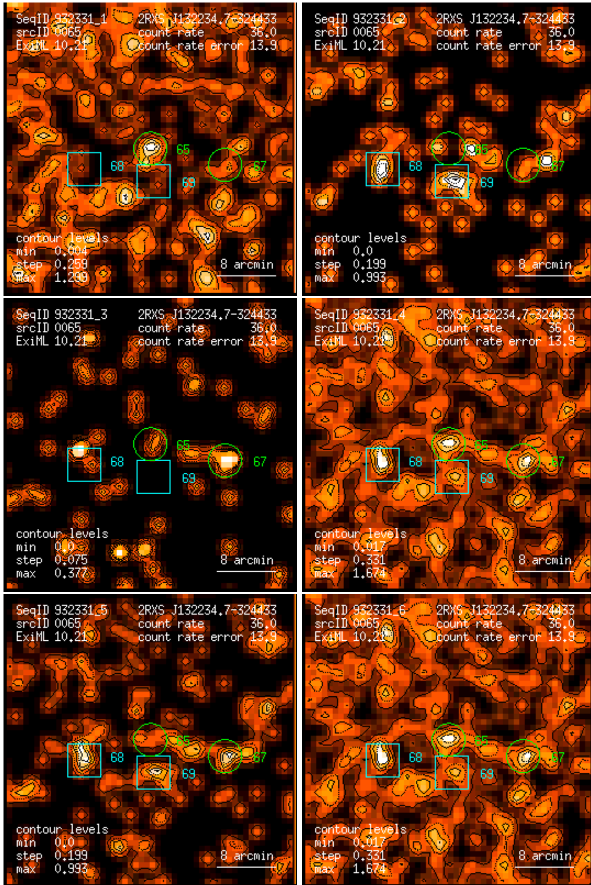
Figure 65: RASS 932331: detection 0065: band rate images, Gaussian filter: (1) PSPC channels 11 – 41, (2) 52 – 90, (3) 91 – 201, (4) 11 – 235, (5) 52 – 201, (6) 11 – 201. Broad band rates in counts/ks. Band rate contour levels in counts/ks/arcmin 2 .
