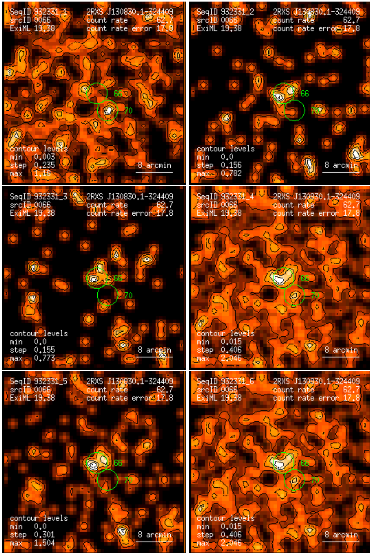
Figure 66: RASS 932331: detection 0066: band rate images, Gaussian filter: (1) PSPC channels 11 – 41, (2) 52 – 90, (3) 91 – 201, (4) 11 – 235, (5) 52 – 201, (6) 11 – 201. Broad band rates in counts/ks. Band rate contour levels in counts/ks/arcmin 2 .
