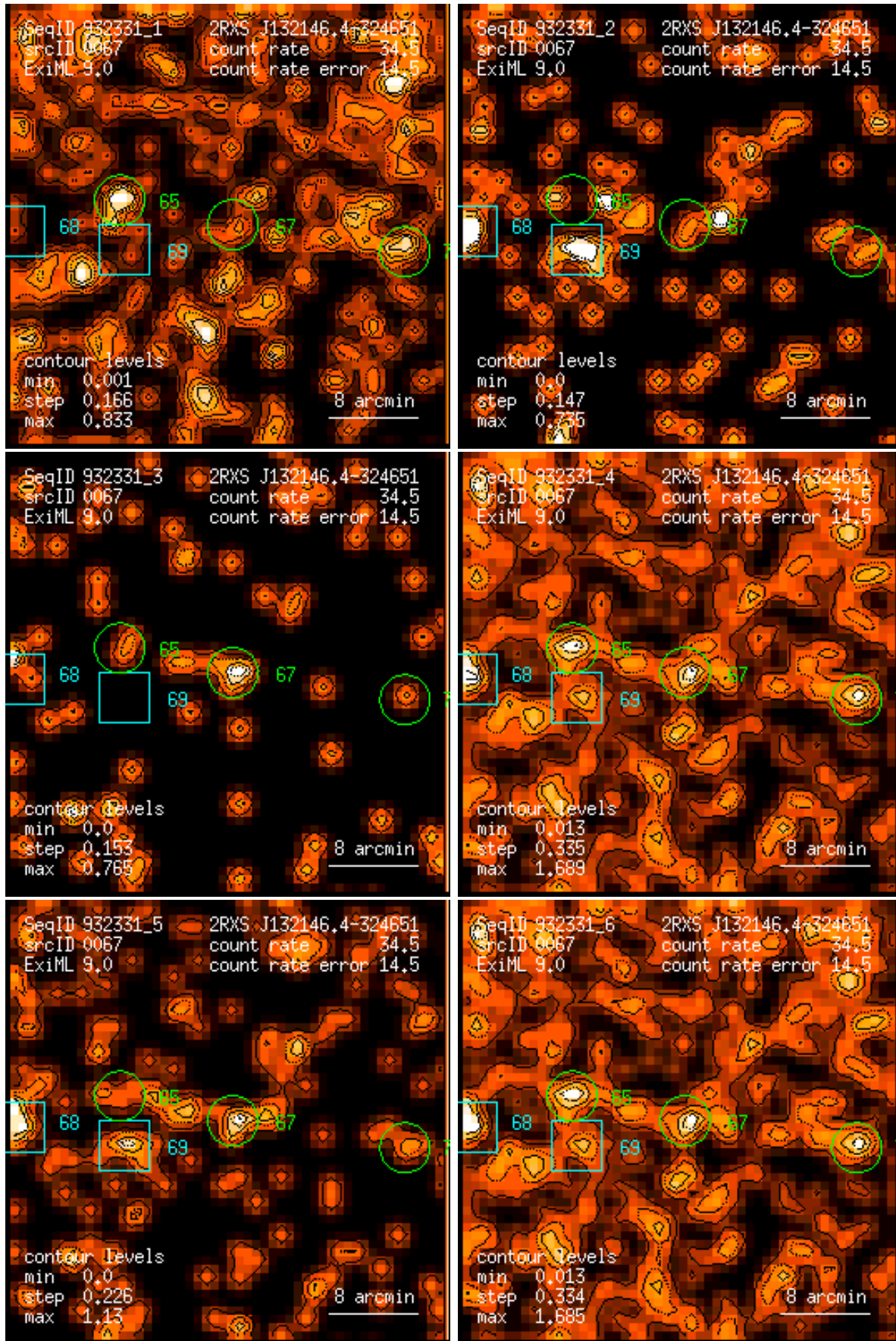
Figure 67: RASS 932331: detection 0067: band rate images, Gaussian filter: (1) PSPC channels 11 – 41, (2) 52 – 90, (3) 91 – 201, (4) 11 – 235, (5) 52 – 201, (6) 11 – 201. Broad band rates in counts/ks. Band rate contour levels in counts/ks/arcmin 2 .
