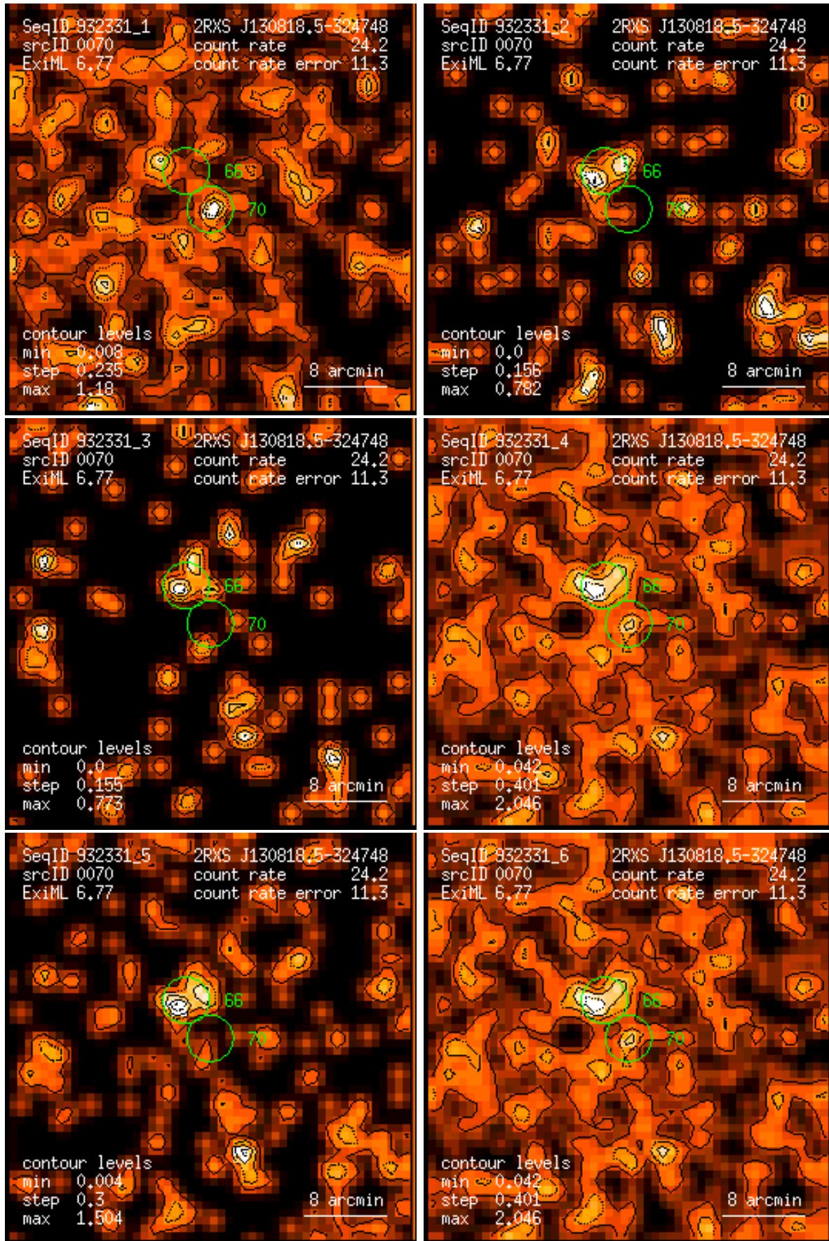
Figure 70: RASS 932331: detection 0070: band rate images, Gaussian filter: (1) PSPC channels 11 – 41, (2) 52 – 90, (3) 91 – 201, (4) 11 – 235, (5) 52 – 201, (6) 11 – 201. Broad band rates in counts/ks. Band rate contour levels in counts/ks/arcmin 2 .
