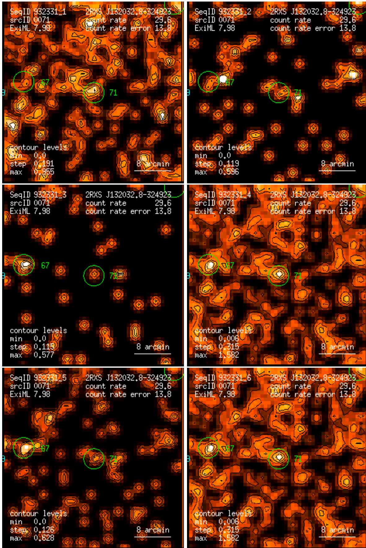
Figure 71: RASS 932331: detection 0071: band rate images, Gaussian filter: (1) PSPC channels 11 – 41, (2) 52 – 90, (3) 91 – 201, (4) 11 – 235, (5) 52 – 201, (6) 11 – 201. Broad band rates in counts/ks. Band rate contour levels in counts/ks/arcmin 2 .
