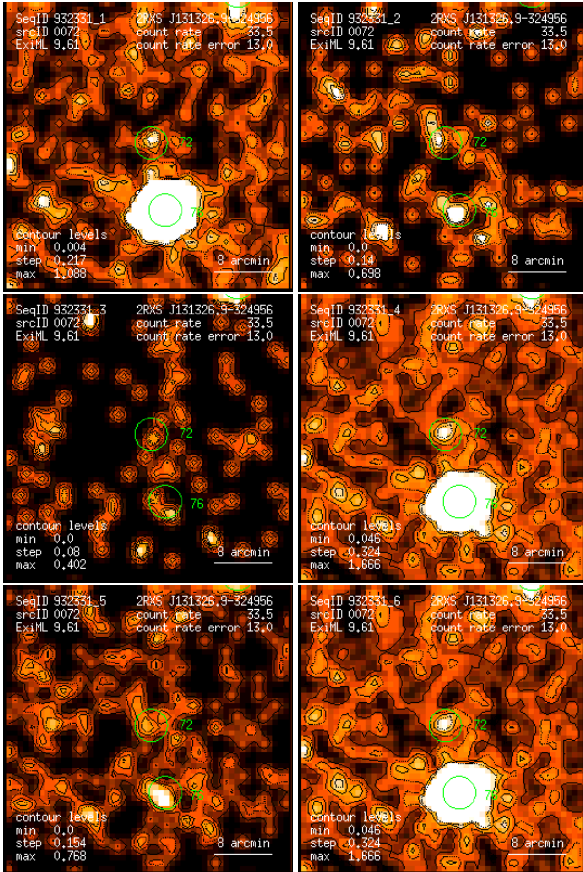
Figure 72: RASS 932331: detection 0072: band rate images, Gaussian filter: (1) PSPC channels 11 – 41, (2) 52 – 90, (3) 91 – 201, (4) 11 – 235, (5) 52 – 201, (6) 11 – 201. Broad band rates in counts/ks. Band rate contour levels in counts/ks/arcmin 2 .
