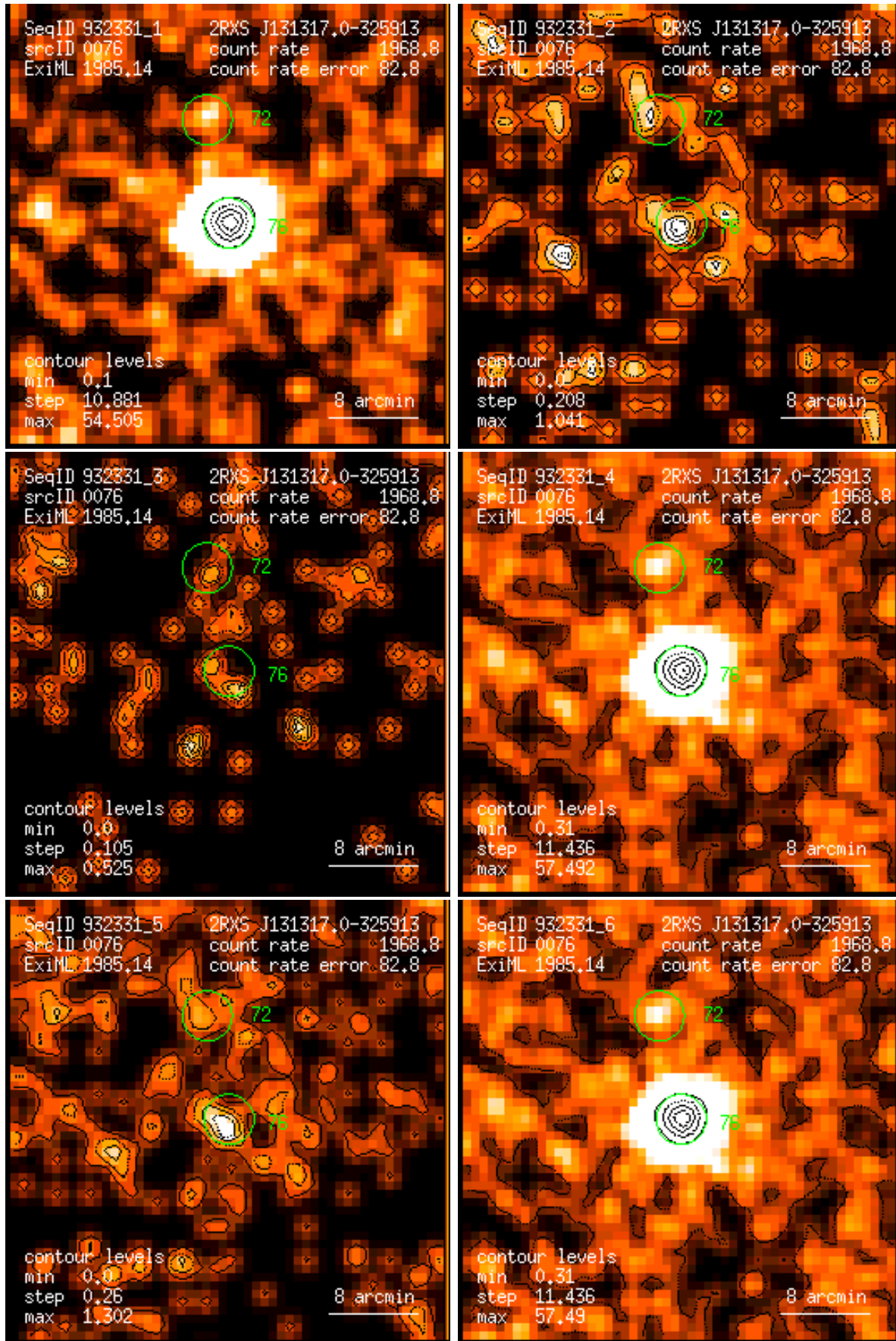
Figure 76: RASS 932331: detection 0076: band rate images, Gaussian filter: (1) PSPC channels 11 – 41, (2) 52 – 90, (3) 91 – 201, (4) 11 – 235, (5) 52 – 201, (6) 11 – 201. Broad band rates in counts/ks. Band rate contour levels in counts/ks/arcmin 2 .
