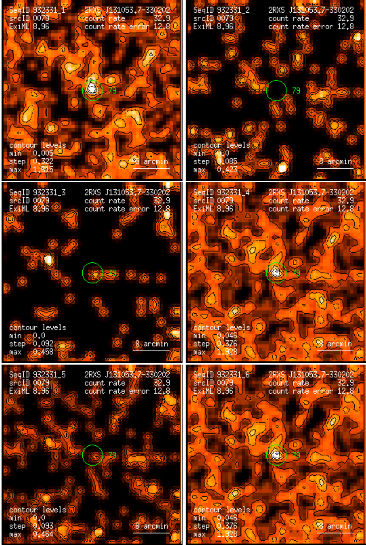
Figure 79: RASS 932331: detection 0079: band rate images, Gaussian filter: (1) PSPC channels 11 – 41, (2) 52 – 90, (3) 91 – 201, (4) 11 – 235, (5) 52 – 201, (6) 11 – 201. Broad band rates in counts/ks. Band rate contour levels in counts/ks/arcmin 2 .
