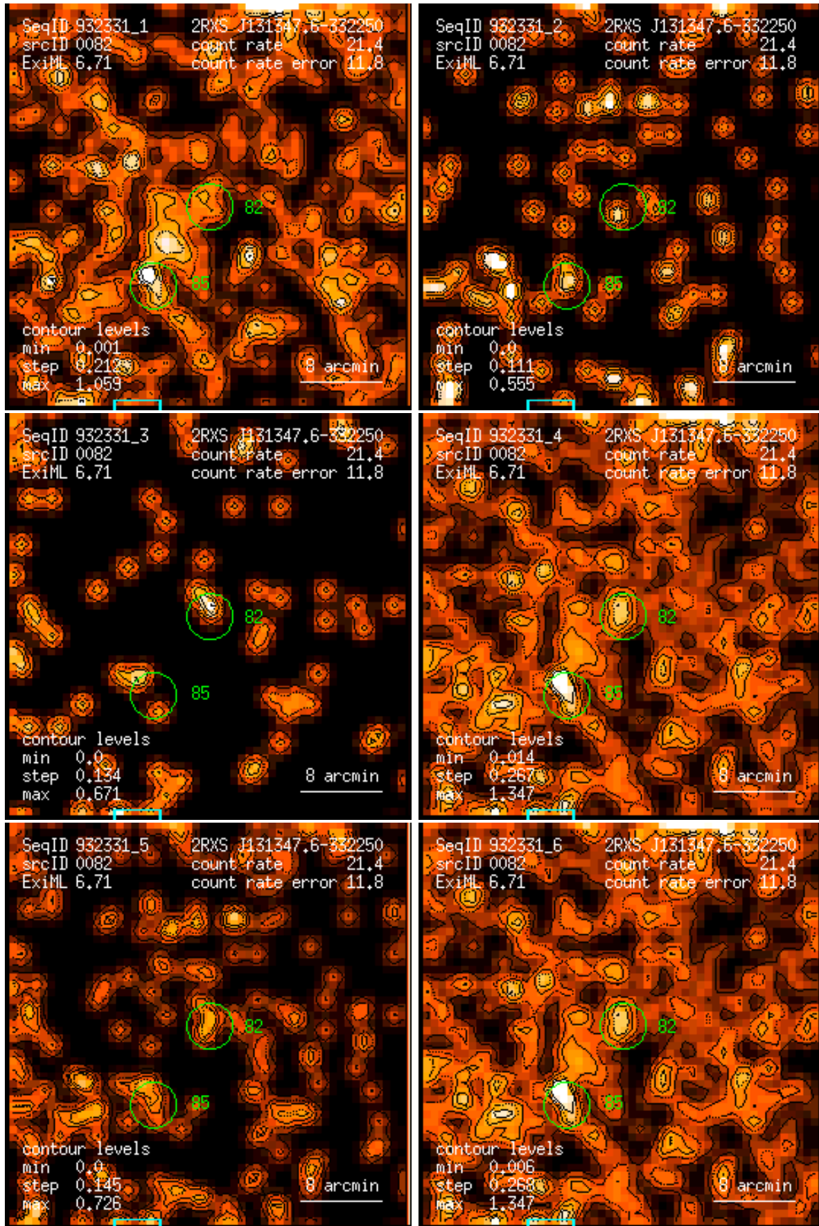
Figure 82: RASS 932331: detection 0082: band rate images, Gaussian filter: (1) PSPC channels 11 – 41, (2) 52 – 90, (3) 91 – 201, (4) 11 – 235, (5) 52 – 201, (6) 11 – 201. Broad band rates in counts/ks. Band rate contour levels in counts/ks/arcmin 2 .
