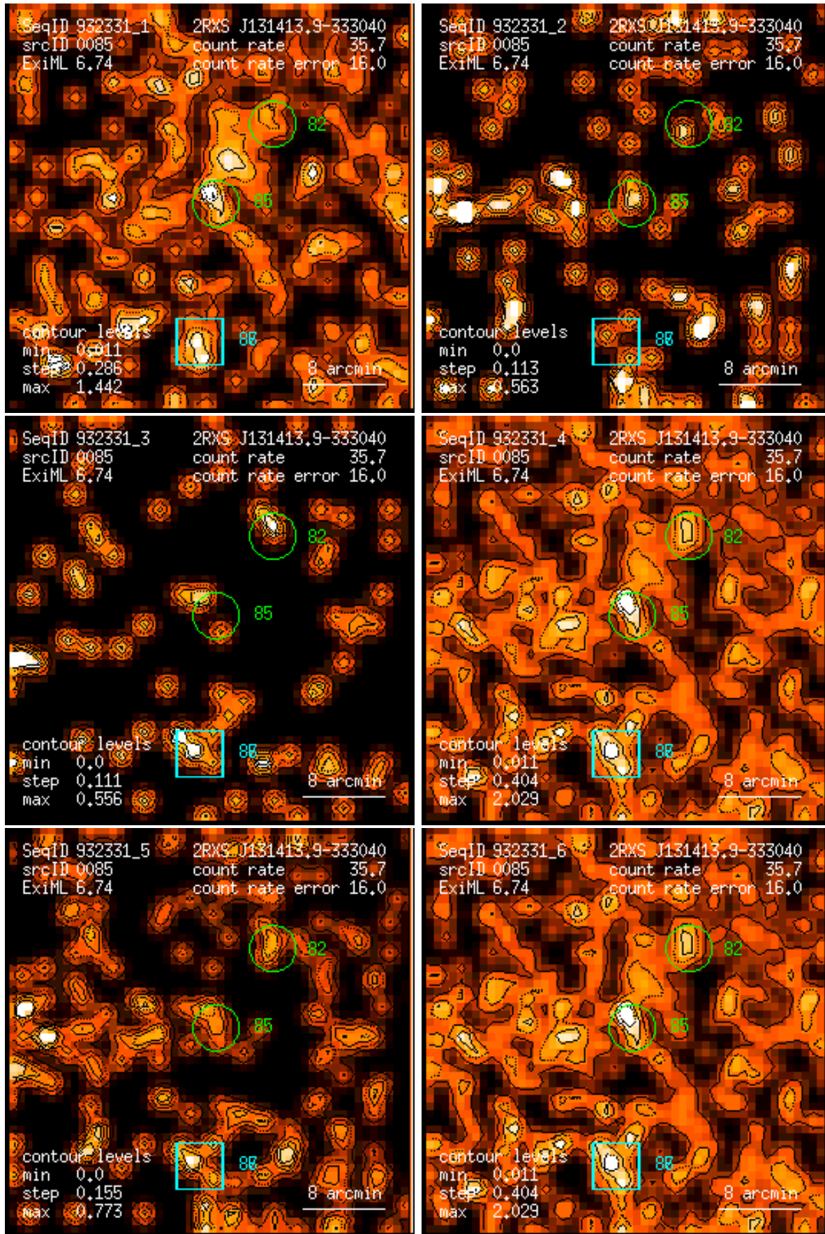
Figure 85: RASS 932331: detection 0085: band rate images, Gaussian filter: (1) PSPC channels 11 – 41, (2) 52 – 90, (3) 91 – 201, (4) 11 – 235, (5) 52 – 201, (6) 11 – 201. Broad band rates in counts/ks. Band rate contour levels in counts/ks/arcmin 2 .
