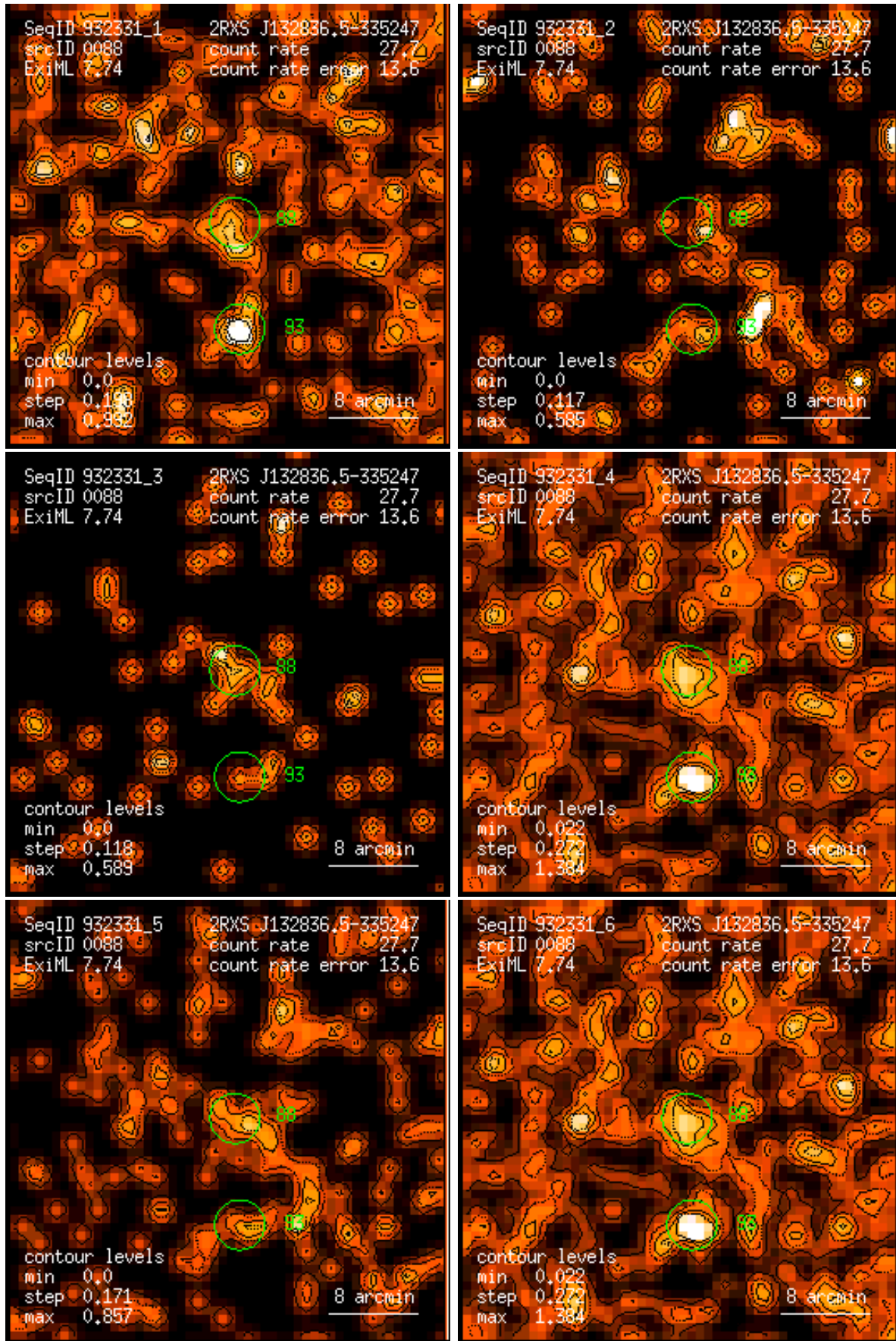
Figure 88: RASS 932331: detection 0088: band rate images, Gaussian filter: (1) PSPC channels 11 – 41, (2) 52 – 90, (3) 91 – 201, (4) 11 – 235, (5) 52 – 201, (6) 11 – 201. Broad band rates in counts/ks. Band rate contour levels in counts/ks/arcmin 2 .
