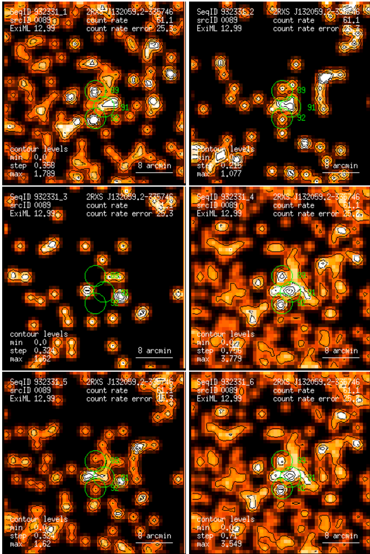
Figure 89: RASS 932331: detection 0089: band rate images, Gaussian filter: (1) PSPC channels 11 – 41, (2) 52 – 90, (3) 91 – 201, (4) 11 – 235, (5) 52 – 201, (6) 11 – 201. Broad band rates in counts/ks. Band rate contour levels in counts/ks/arcmin 2 .
