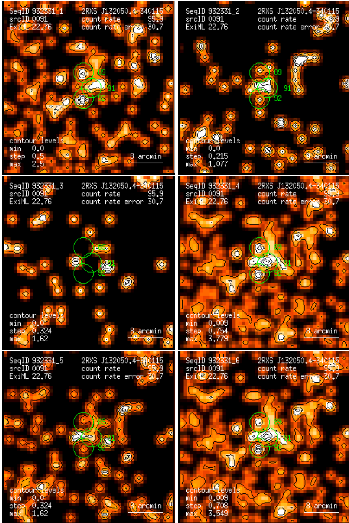
Figure 91: RASS 932331: detection 0091: band rate images, Gaussian filter: (1) PSPC channels 11 – 41, (2) 52 – 90, (3) 91 – 201, (4) 11 – 235, (5) 52 – 201, (6) 11 – 201. Broad band rates in counts/ks. Band rate contour levels in counts/ks/arcmin 2 .
