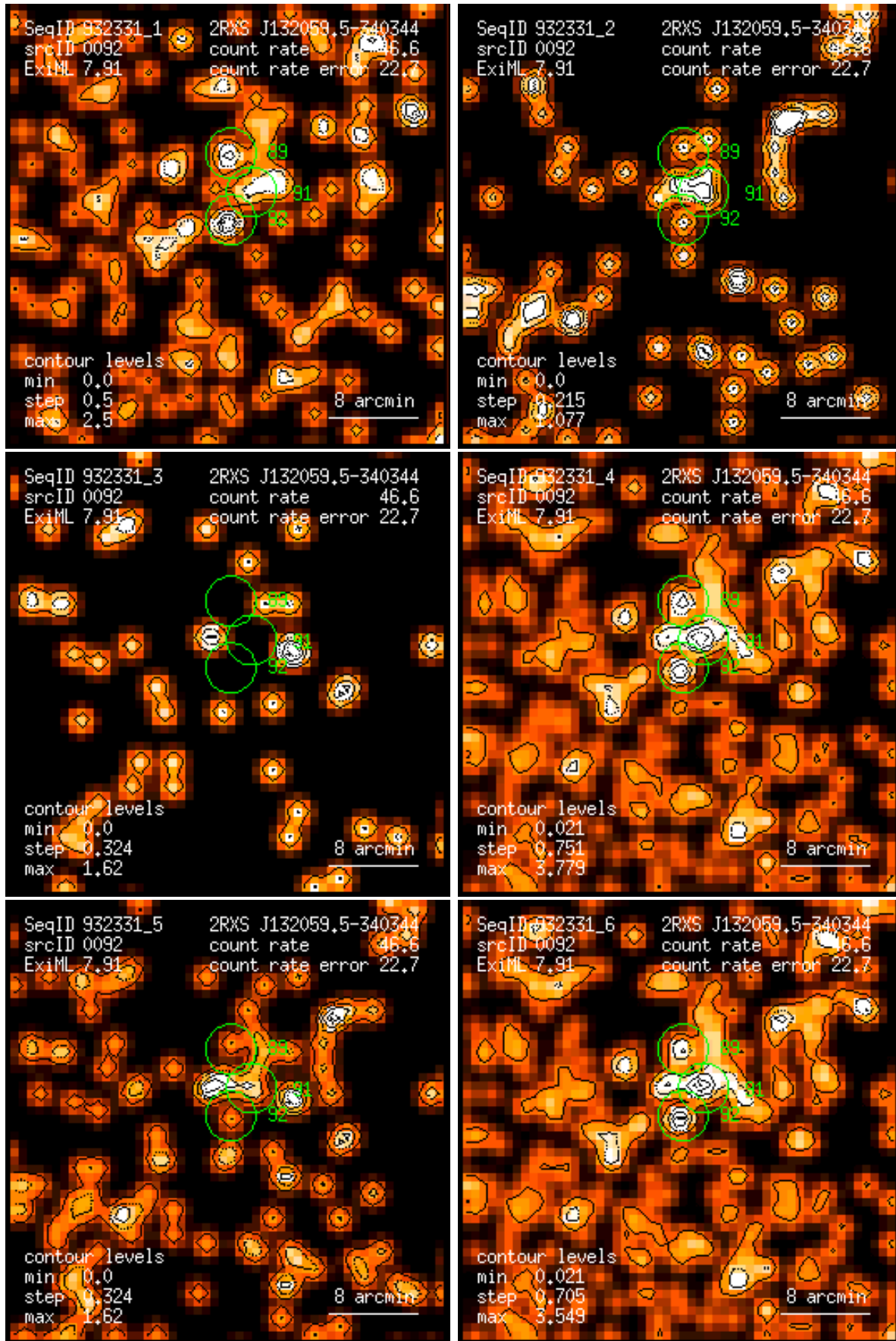
Figure 92: RASS 932331: detection 0092: band rate images, Gaussian filter: (1) PSPC channels 11 – 41, (2) 52 – 90, (3) 91 – 201, (4) 11 – 235, (5) 52 – 201, (6) 11 – 201. Broad band rates in counts/ks. Band rate contour levels in counts/ks/arcmin 2 .
