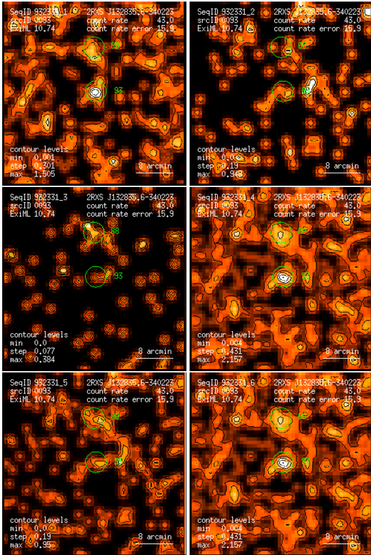
Figure 93: RASS 932331: detection 0093: band rate images, Gaussian filter: (1) PSPC channels 11 – 41, (2) 52 – 90, (3) 91 – 201, (4) 11 – 235, (5) 52 – 201, (6) 11 – 201. Broad band rates in counts/ks. Band rate contour levels in counts/ks/arcmin 2 .
