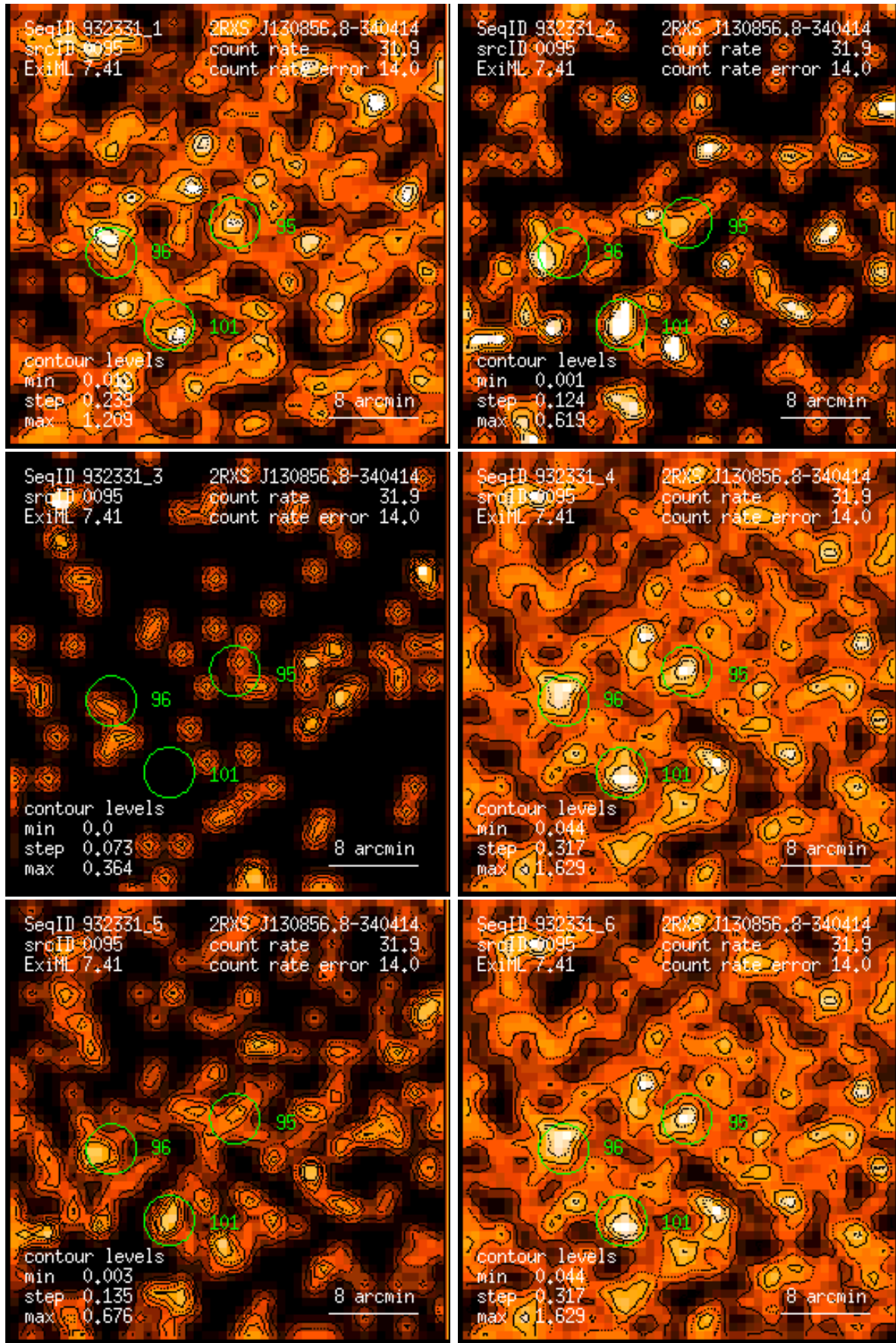
Figure 95: RASS 932331: detection 0095: band rate images, Gaussian filter: (1) PSPC channels 11 – 41, (2) 52 – 90, (3) 91 – 201, (4) 11 – 235, (5) 52 – 201, (6) 11 – 201. Broad band rates in counts/ks. Band rate contour levels in counts/ks/arcmin 2 .
