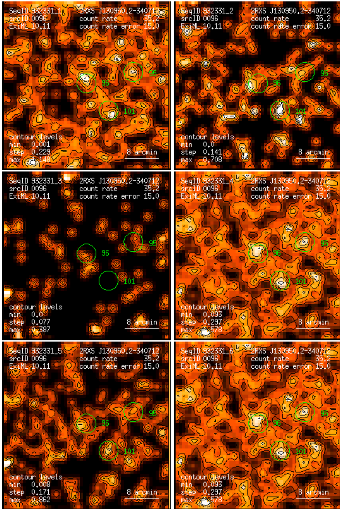
Figure 96: RASS 932331: detection 0096: band rate images, Gaussian filter: (1) PSPC channels 11 – 41, (2) 52 – 90, (3) 91 – 201, (4) 11 – 235, (5) 52 – 201, (6) 11 – 201. Broad band rates in counts/ks. Band rate contour levels in counts/ks/arcmin 2 .
