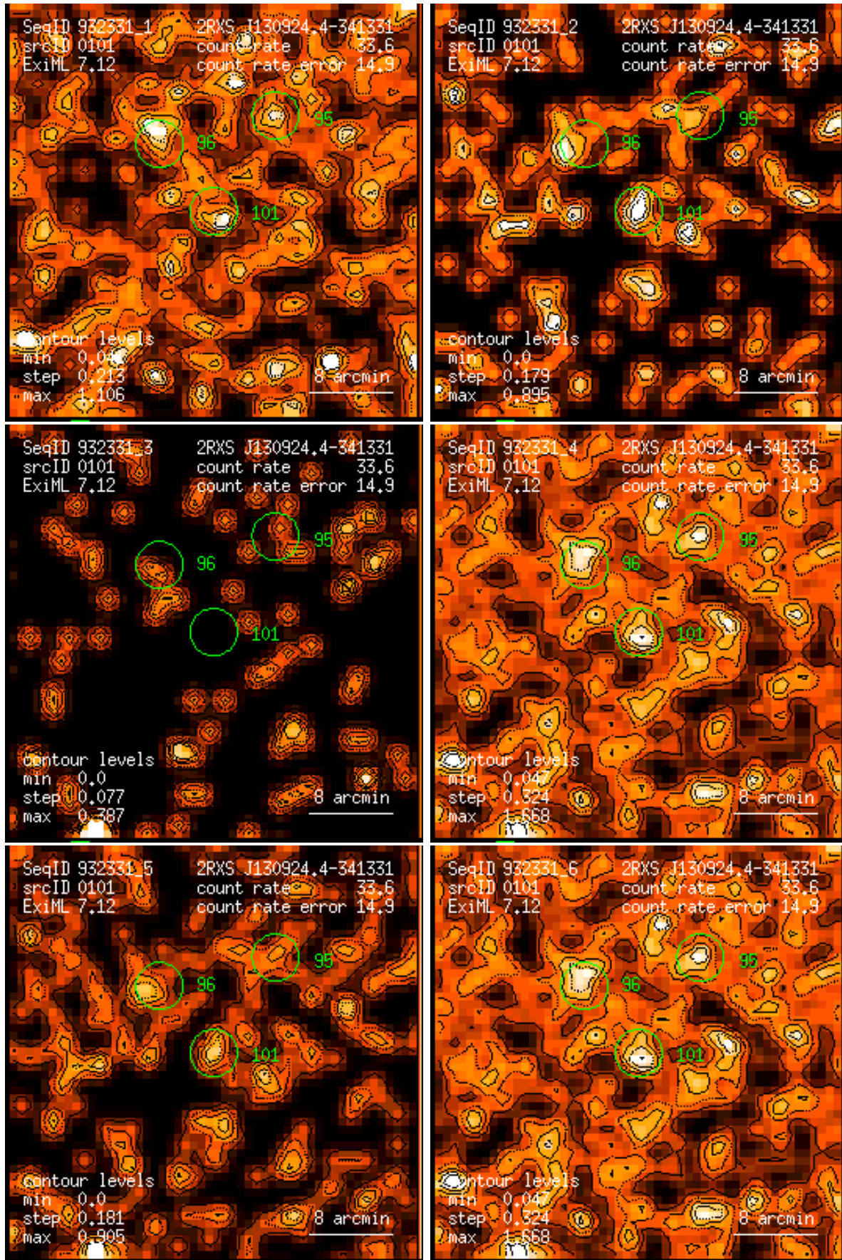
Figure 101: RASS 932331: detection 0101: band rate images, Gaussian filter: (1) PSPC channels 11 – 41, (2) 52 – 90, (3) 91 – 201, (4) 11 – 235, (5) 52 – 201, (6) 11 – 201. Broad band rates in counts/ks. Band rate contour levels in counts/ks/arcmin 2 .
