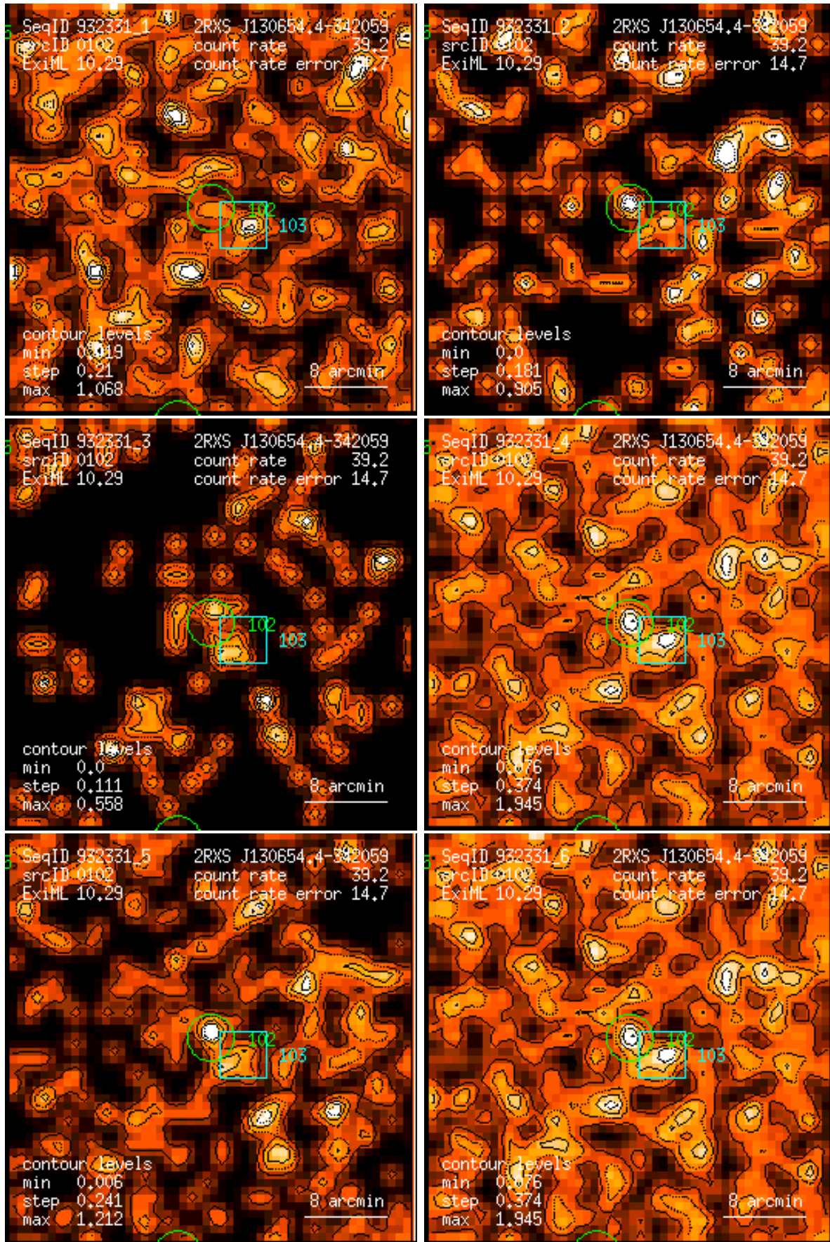
Figure 102: RASS 932331: detection 0102: band rate images, Gaussian filter: (1) PSPC channels 11 – 41, (2) 52 – 90, (3) 91 – 201, (4) 11 – 235, (5) 52 – 201, (6) 11 – 201. Broad band rates in counts/ks. Band rate contour levels in counts/ks/arcmin 2 .
