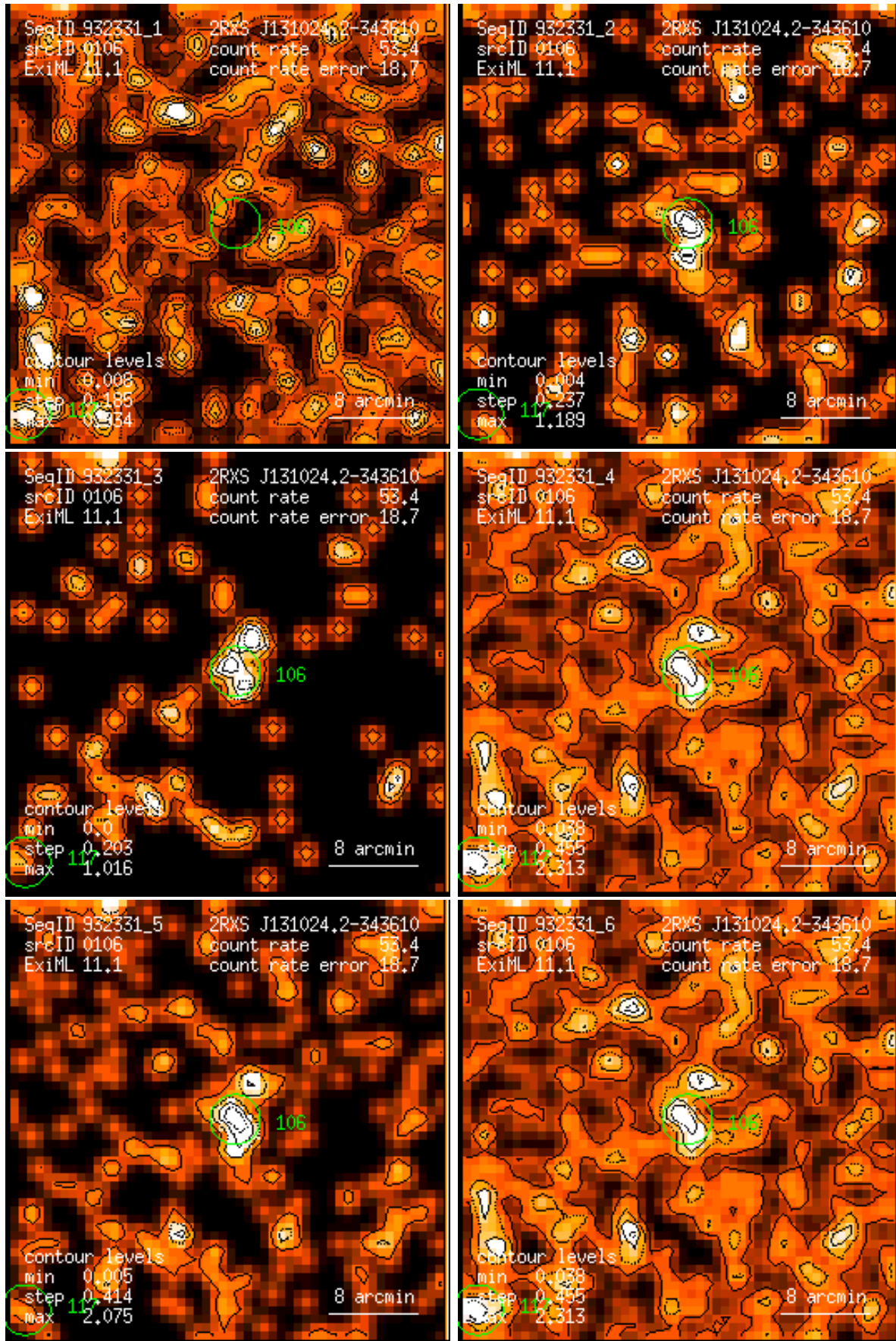
Figure 106: RASS 932331: detection 0106: band rate images, Gaussian filter: (1) PSPC channels 11 – 41, (2) 52 – 90, (3) 91 – 201, (4) 11 – 235, (5) 52 – 201, (6) 11 – 201. Broad band rates in counts/ks. Band rate contour levels in counts/ks/arcmin 2 .
