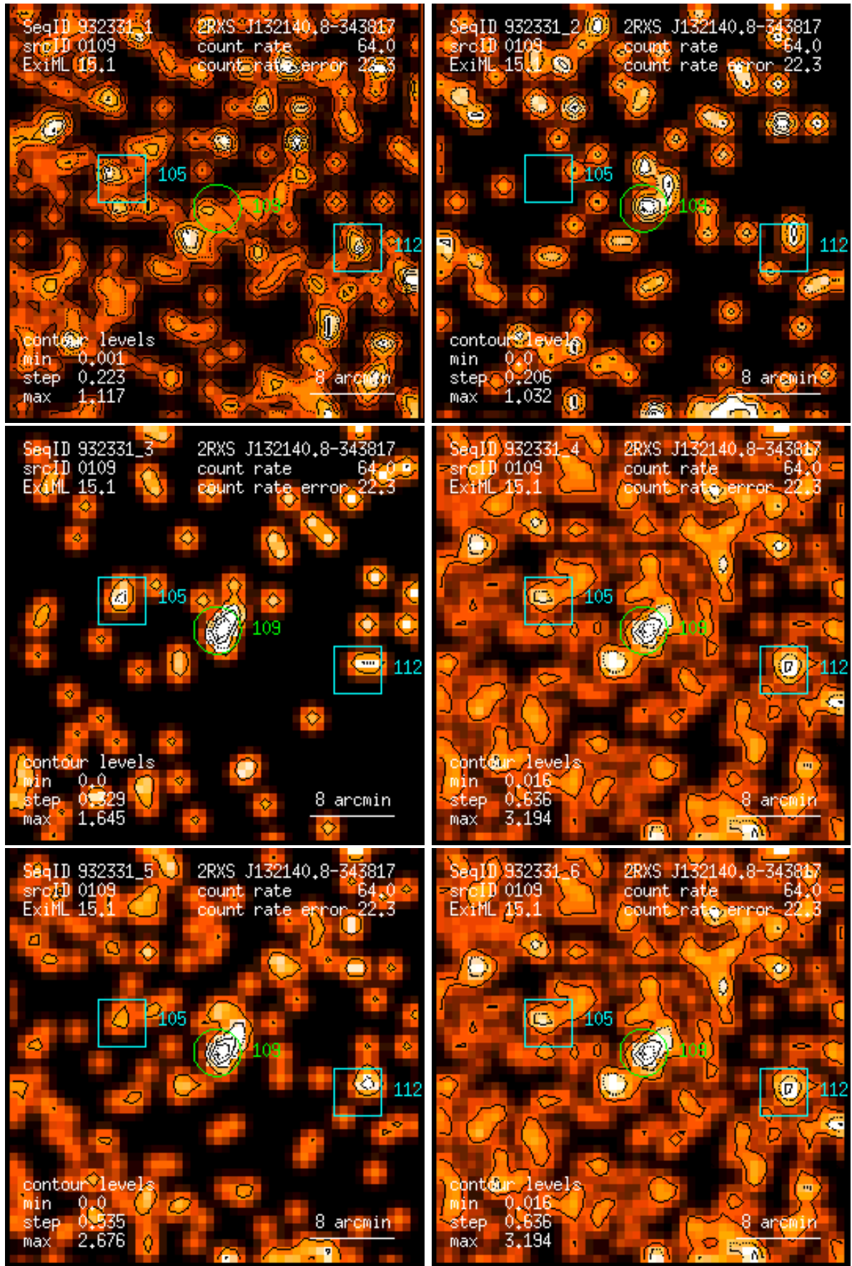
Figure 109: RASS 932331: detection 0109: band rate images, Gaussian filter: (1) PSPC channels 11 – 41, (2) 52 – 90, (3) 91 – 201, (4) 11 – 235, (5) 52 – 201, (6) 11 – 201. Broad band rates in counts/ks. Band rate contour levels in counts/ks/arcmin 2 .
