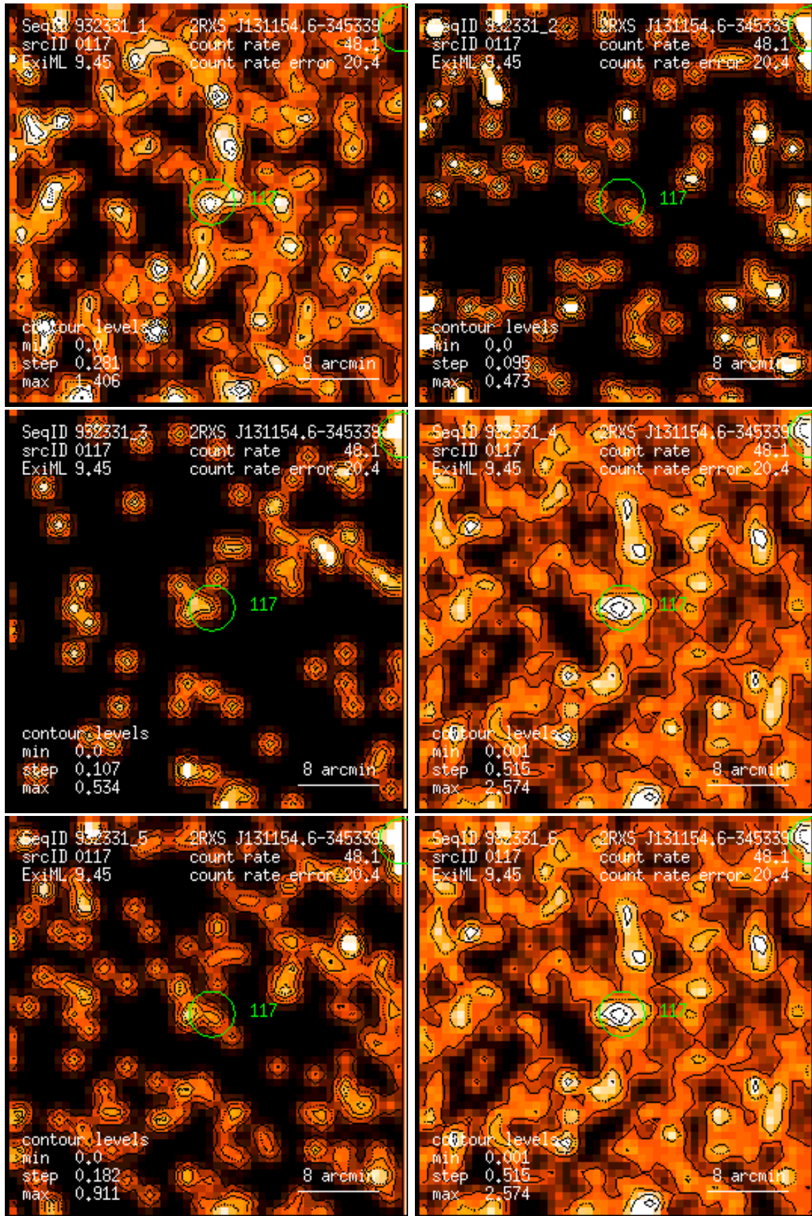
Figure 117: RASS 932331: detection 0117: band rate images, Gaussian filter: (1) PSPC channels 11 – 41, (2) 52 – 90, (3) 91 – 201, (4) 11 – 235, (5) 52 – 201, (6) 11 – 201. Broad band rates in counts/ks. Band rate contour levels in counts/ks/arcmin 2 .
