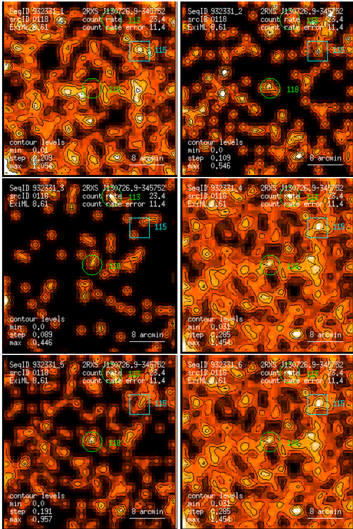
Figure 118: RASS 932331: detection 0118: band rate images, Gaussian filter: (1) PSPC channels 11 – 41, (2) 52 – 90, (3) 91 – 201, (4) 11 – 235, (5) 52 – 201, (6) 11 – 201. Broad band rates in counts/ks. Band rate contour levels in counts/ks/arcmin 2 .
