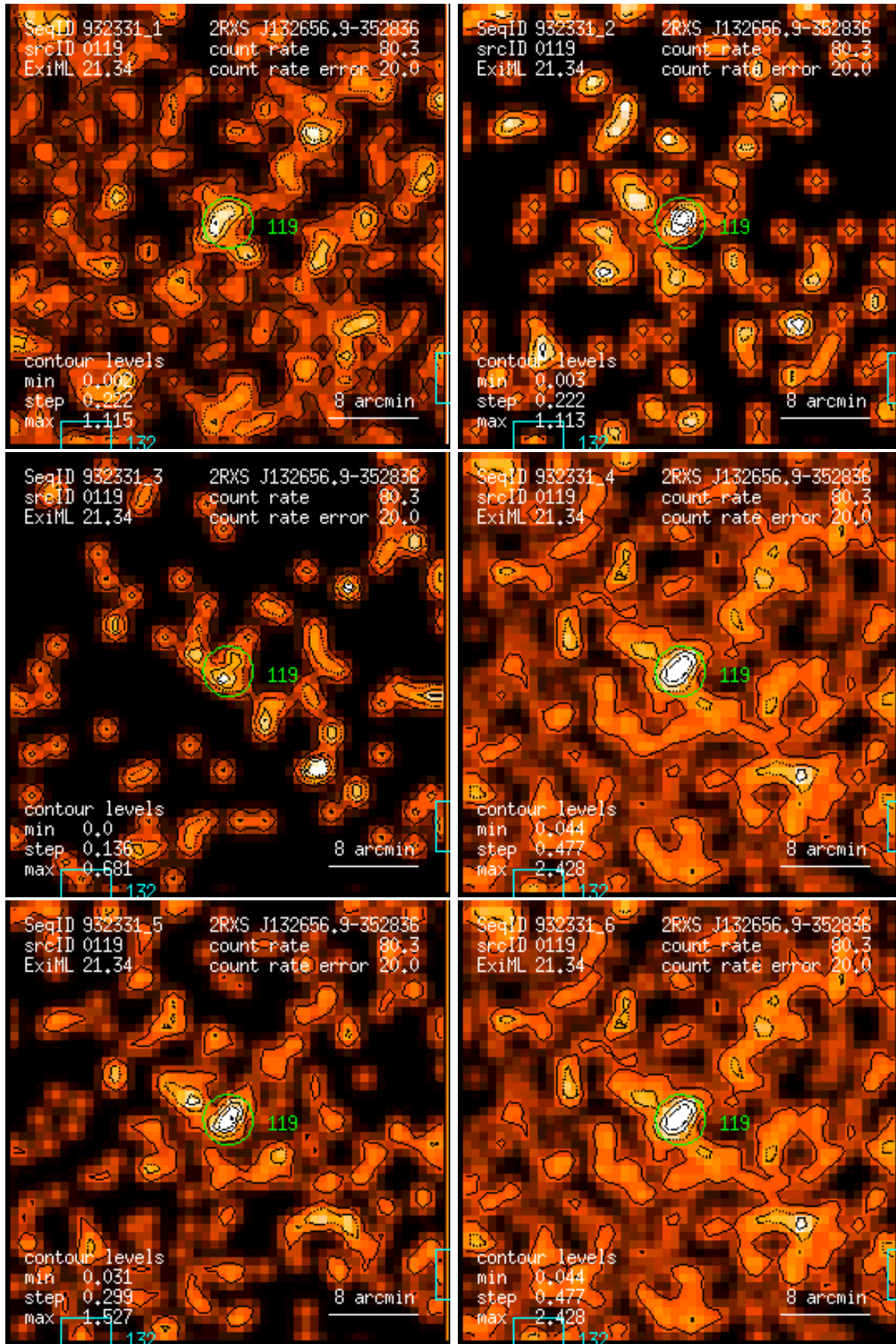
Figure 119: RASS 932331: detection 0119: band rate images, Gaussian filter: (1) PSPC channels 11 – 41, (2) 52 – 90, (3) 91 – 201, (4) 11 – 235, (5) 52 – 201, (6) 11 – 201. Broad band rates in counts/ks. Band rate contour levels in counts/ks/arcmin 2 .
